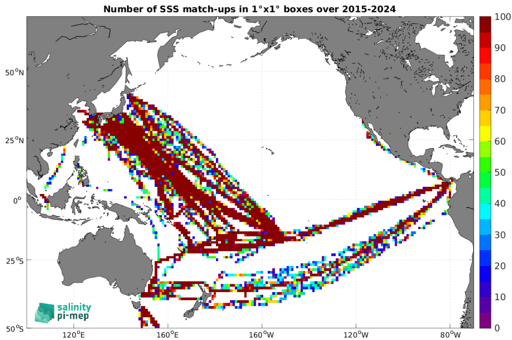
Figure 5: Number of SSS match-ups between TSG (LEGOS-DM) SSS and the SMAP SSS L2 v6 - 40 km (RSS) SSS product for the Pacific Ocean Pi-MEP region over 1^\circ \times 1^\circ boxes and for the full satellite product period.
