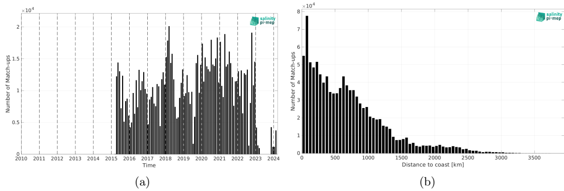
Figure 2: Number of match-ups between TSG (LEGOS-DM) and SMAP SSS L2 v6 - 40 km (RSS) SSS as a function of time (a) and as function of the distance to coast (b) over the Pacific Ocean Pi-MEP region and for the full satellite product period.
