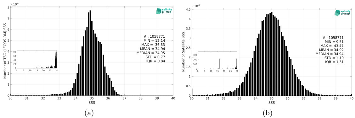
Figure 3: Histograms of SSS from TSG (LEGOS-DM) (a) and SMAP SSS L2 v6 - 40 km (RSS) (b) considering all match-up pairs per bins of 0.1 over the Pacific Ocean Pi-MEP region and for the full satellite product period.
