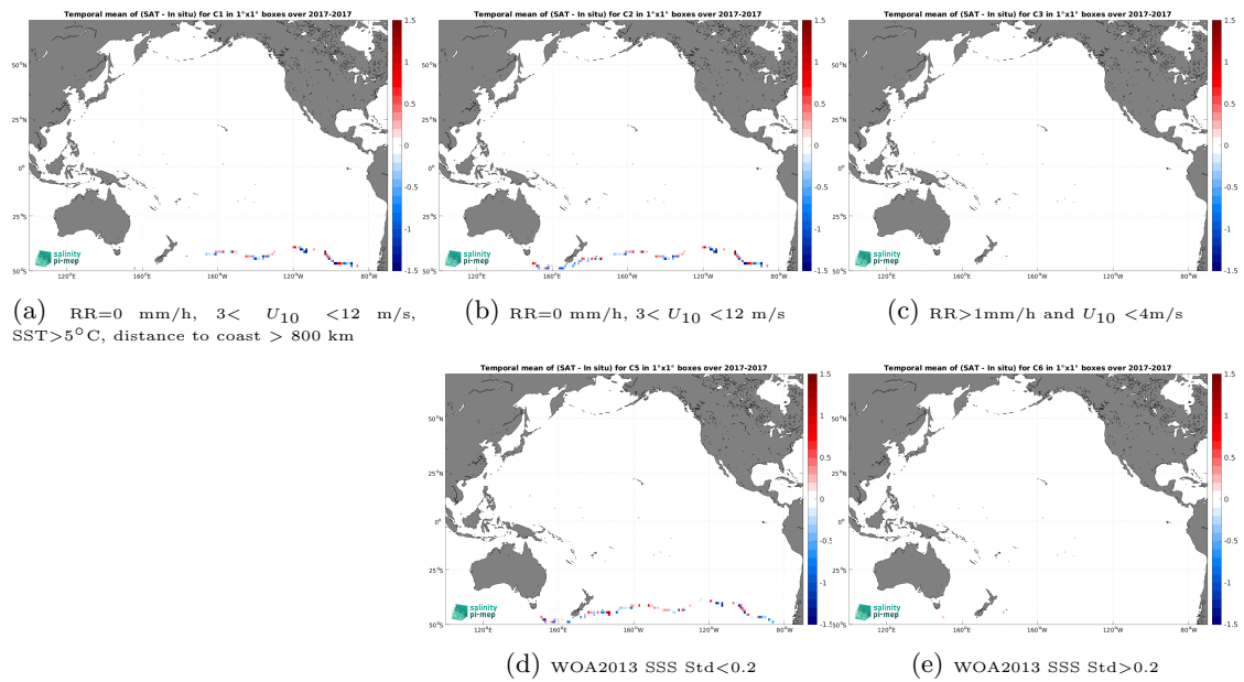
Figure 14: Temporal mean gridded over spatial boxes of size 1^\circ \times 1^\circ of \Delta SSS (SMAP SSS L2 v6 - 40 km (RSS) - TSG (GOSUD-Sailing-ship)) for 5 different subdatasets corresponding to: RR=0 mm/h, 3 < U_{10} < 12 m/s, SST > 5°C, distance to coast > 800 km (a), RR=0 mm/h, 3 < U_{10} < 12 m/s (b), RR > 1mm/h and U_{10} < 4 m/s (c), WOA2013 SSS Std < 0.2 (d), WOA2013 SSS Std > 0.2 (e).
