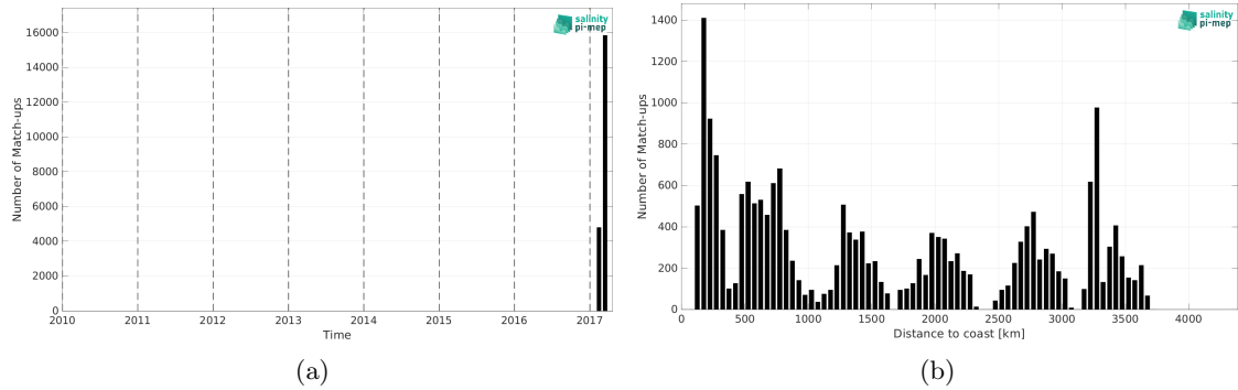
Figure 2: Number of match-ups between TSG (GOSUD-Sailing-ship) and SMAP SSS L2 v6 - 40 km (RSS) SSS as a function of time (a) and as function of the distance to coast (b) over the Pacific Ocean Pi-MEP region and for the full satellite product period.
