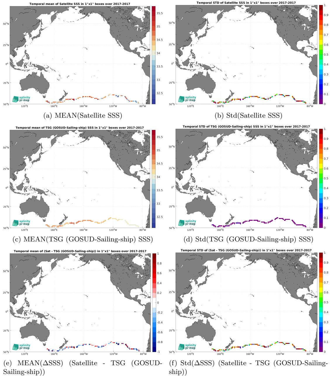
Figure 7: Temporal mean (left) and Std (right) of SSS from SMAP SSS L2 v6 - 40 km (RSS) (top), TSG (GOSUD-Sailing-ship) (middle), and of \Delta SSS (Satellite - TSG (GOSUD-Sailing-ship)). Only match-up pairs are used to generate these maps.
