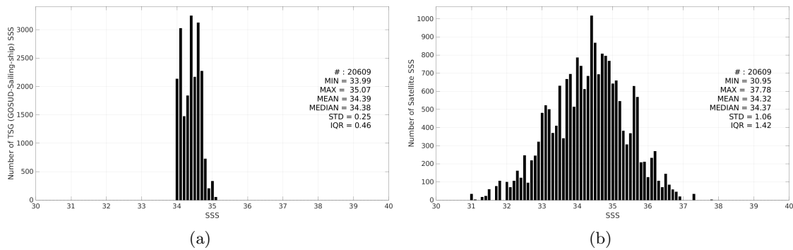
Figure 3: Histograms of SSS from TSG (GOSUD-Sailing-ship) (a) and SMAP SSS L2 v6 - 40 km (RSS) (b) considering all match-up pairs per bins of 0.1 over the Pacific Ocean Pi-MEP region and for the full satellite product period.
