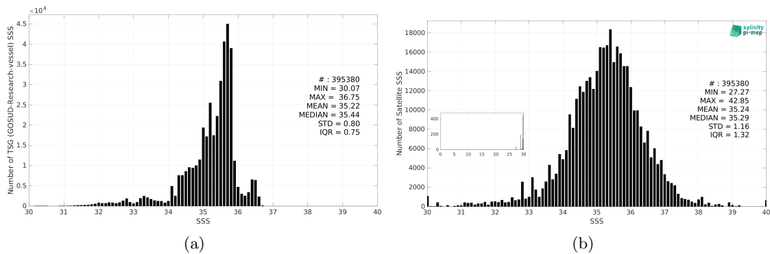
Figure 3: Histograms of SSS from TSG (GOSUD-Research-vessel) (a) and SMAP SSS L2 v6 - 40 km (RSS) (b) considering all match-up pairs per bins of 0.1 over the Pacific Ocean Pi-MEP region and for the full satellite product period.
