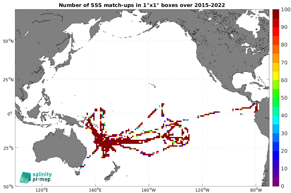
Figure 5: Number of SSS match-ups between TSG (GOSUD-Research-vessel) SSS and the SMAP SSS L2 v6 - 40 km (RSS) SSS product for the Pacific Ocean Pi-MEP region over 1°x1° boxes and for the full satellite product period.
