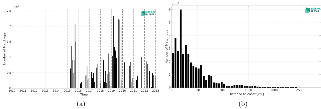
Figure 2: Number of match-ups between TSG (GOSUD-Research-vessel) and SMAP SSS L2 v6 - 40 km (RSS) SSS as a function of time (a) and as function of the distance to coast (b) over the Pacific Ocean Pi-MEP region and for the full satellite product period.
