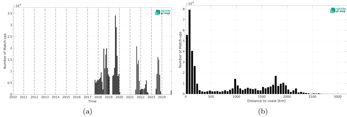
Figure 2: Number of match-ups between Saildrone and SMAP SSS L2 v6 - 40 km (RSS) SSS as a function of time (a) and as function of the distance to coast (b) over the Pacific Ocean Pi-MEP region and for the full satellite product period.
