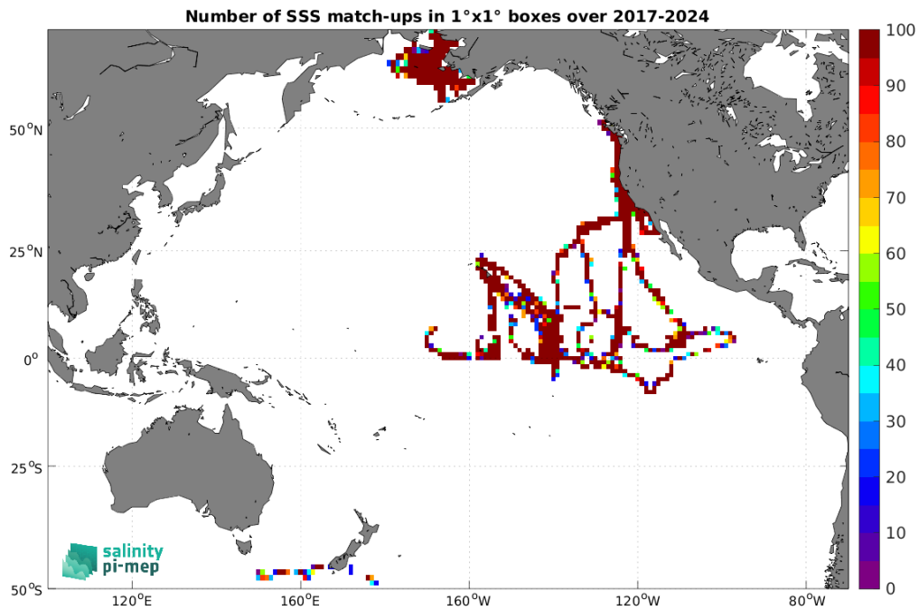
Figure 5: Number of SSS match-ups between Sairdron SSS and the SMAP SSS L2 v6 - 40 km (RSS) SSS product for the Pacific Ocean Pi-MEP region over 1^\circ \times 1^\circ boxes and for the full satellite product period.
