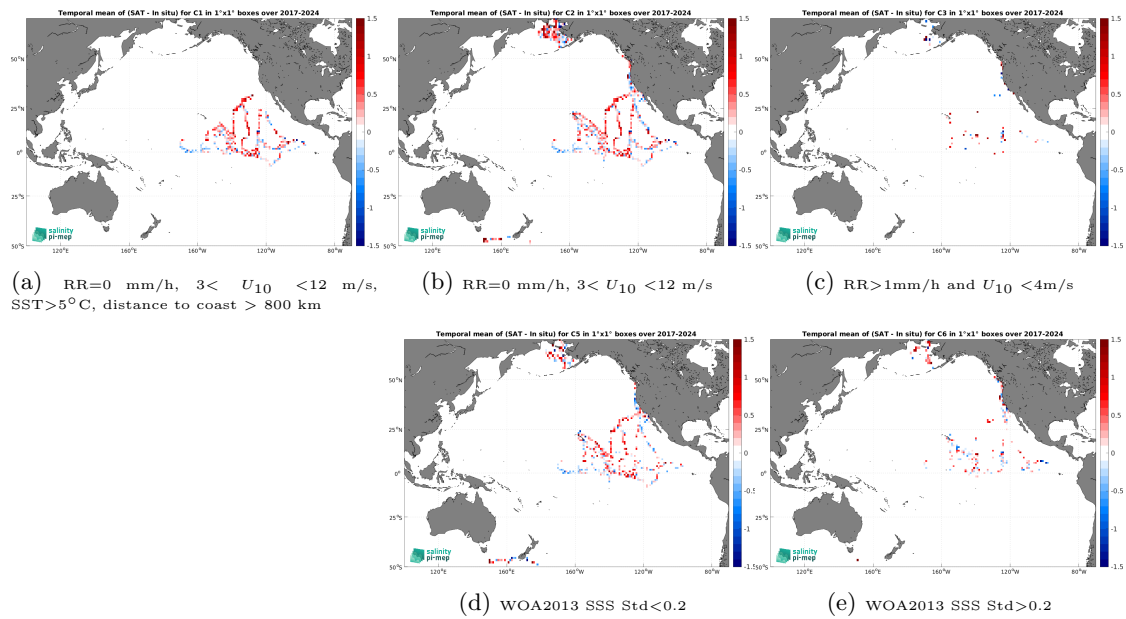
Figure 14: Temporal mean gridded over spatial boxes of size 1^\circ \times 1^\circ of \Delta SSS (SMAP SSS L2 v6 - 40 km (RSS) - Sairdrone) for 5 different subdatasets corresponding to:RR=0 mm/h, 3 < U_{10} < 12 m/s, SST > 5^\circ\text{C} , distance to coast > 800 km (a), RR=0 mm/h, 3 < U_{10} < 12 m/s (b), RR > 1 mm/h and U_{10} < 4 m/s (c), WOA2013 SSS Std < 0.2 (d), WOA2013 SSS Std > 0.2 (e).
