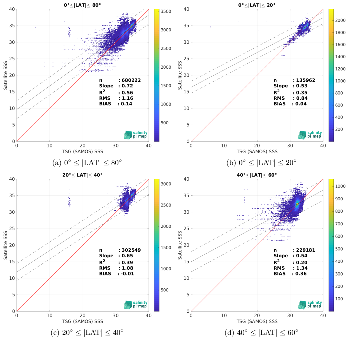
Figure 9: Contour maps of the concentration of SMAP SSS L2 v5 (RSS) SSS (y-axis) versus TSG (SAMOS) SSS (x-axis) at match-up pairs for different latitude bands. For each plot, the red line shows x=y . The black thin and dashed lines indicate a linear fit through the data cloud and the \pm 95\% confidence levels, respectively. The number match-up pairs n , the slope and R^2 coefficient of the linear fit, the root mean square (RMS) and the mean bias between satellite and in situ data are indicated for each latitude band in each plots.
