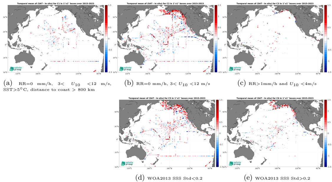
Figure 12: Temporal mean gridded over spatial boxes of size 1^\circ \times 1^\circ of \Delta\text{SSS} (SMAP SSS L2 v5 (RSS) - TSG (SAMOS)) for 5 different subdatasets corresponding to:RR=0 mm/h, 3 < U_{10} < 12 m/s, SST >5^\circ\text{C} , distance to coast > 800 km (a), RR=0 mm/h, 3 < U_{10} < 12 m/s (b), RR >1 mm/h and U_{10} < 4 m/s (c), WOA2013 SSS Std <0.2 (d), WOA2013 SSS Std >0.2 (e).
