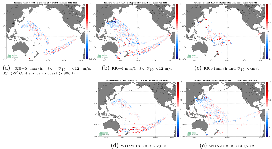
Figure 12: Temporal mean gridded over spatial boxes of size 1^\circ \times 1^\circ of \Delta\text{SSS} (SMAP SSS L2 v5 (RSS) - TSG (LEGOS-DM)) for 5 different subdatasets corresponding to:RR=0 mm/h, 3 < U_{10} < 12 m/s, SST >5^\circ\text{C} , distance to coast > 800 km (a), RR=0 mm/h, 3 < U_{10} < 12 m/s (b), RR >1 mm/h and U_{10} < 4 m/s (c), WOA2013 SSS Std <0.2 (d), WOA2013 SSS Std >0.2 (e).
