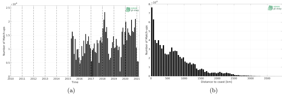
Figure 1: Number of match-ups between TSG (LEGOS-DM) and SMAP SSS L2 v5 (RSS) SSS as a function of time (a) and as function of the distance to coast (b) over the Pacific Ocean Pi-MEP region and for the full satellite product period.
