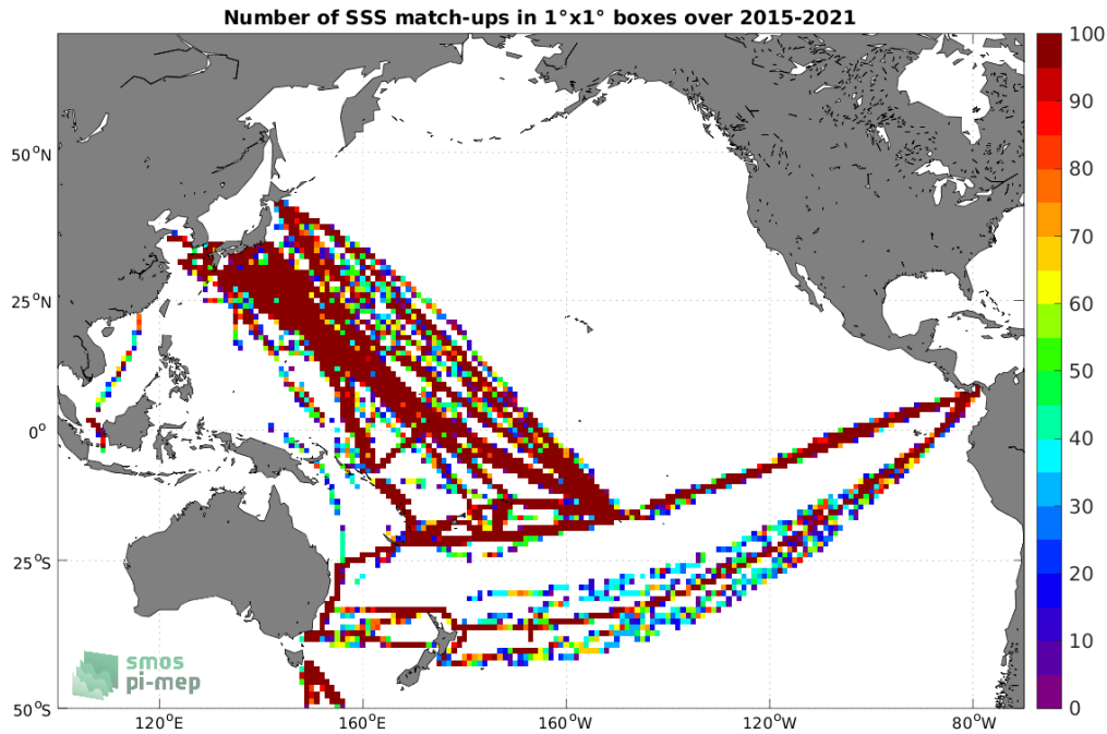
Figure 4: Number of SSS match-ups between TSG (LEGOS-DM) SSS and the SMAP SSS L2 v5 (RSS) SSS product for the Pacific Ocean Pi-MEP region over 1^\circ \times 1^\circ boxes and for the full satellite product period.
