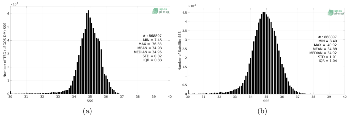
Figure 2: Histograms of SSS from TSG (LEGOS-DM) (a) and SMAP SSS L2 v5 (RSS) (b) considering all match-up pairs per bins of 0.1 over the Pacific Ocean Pi-MEP region and for the full satellite product period.
