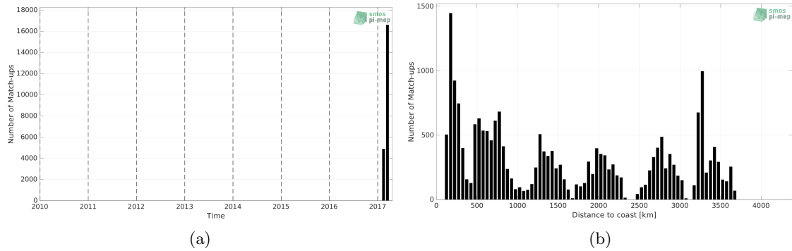
Figure 1: Number of match-ups between TSG (GOSUD-Sailing-ship) and SMAP SSS L2 v5 (RSS) SSS as a function of time (a) and as function of the distance to coast (b) over the Pacific Ocean Pi-MEP region and for the full satellite product period.
