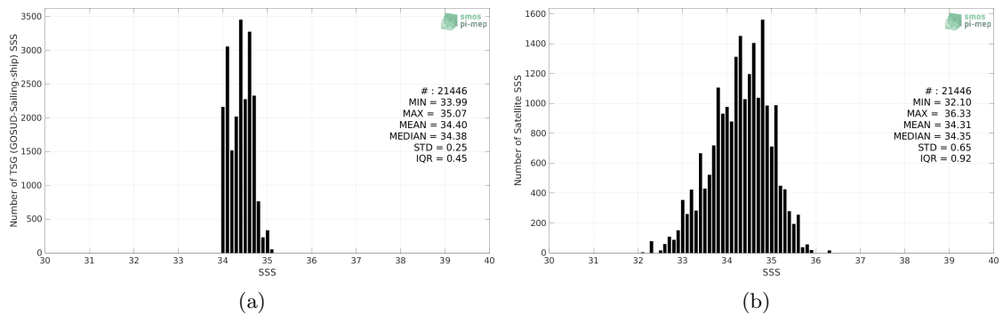
Figure 2: Histograms of SSS from TSG (GOSUD-Sailing-ship) (a) and SMAP SSS L2 v5 (RSS) (b) considering all match-up pairs per bins of 0.1 over the Pacific Ocean Pi-MEP region and for the full satellite product period.
