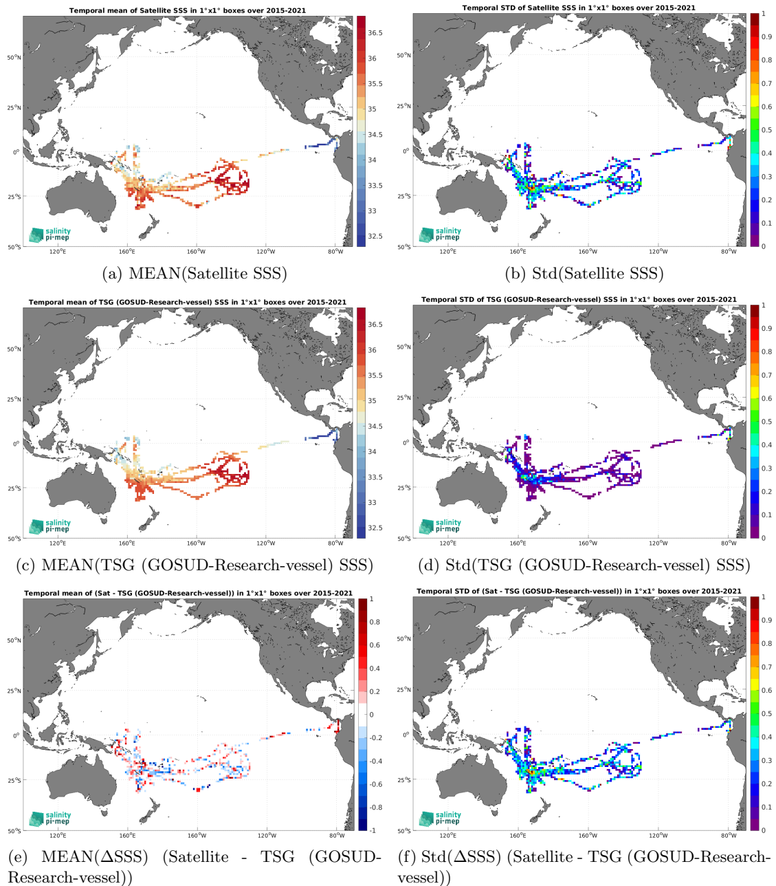
Figure 6: Temporal mean (left) and Std (right) of SSS from SMAP SSS L2 v5 (RSS) (top), TSG (GOSUD-Research-vessel) (middle), and of \Delta SSS (Satellite - TSG (GOSUD-Research-vessel)). Only match-up pairs are used to generate these maps.
