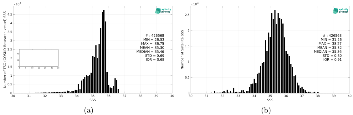
Figure 2: Histograms of SSS from TSG (GOSUD-Research-vessel) (a) and SMAP SSS L2 v5 (RSS) (b) considering all match-up pairs per bins of 0.1 over the Pacific Ocean Pi-MEP region and for the full satellite product period.
