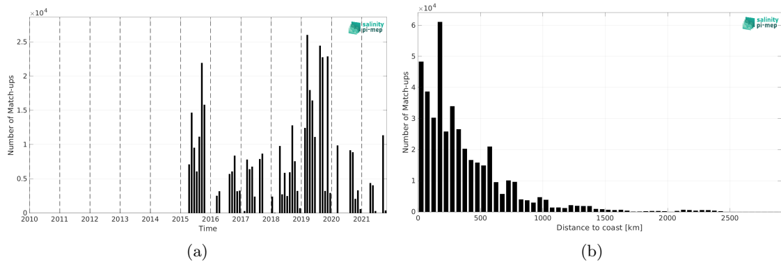
Figure 1: Number of match-ups between TSG (GOSUD-Research-vessel) and SMAP SSS L2 v5 (RSS) SSS as a function of time (a) and as function of the distance to coast (b) over the Pacific Ocean Pi-MEP region and for the full satellite product period.
