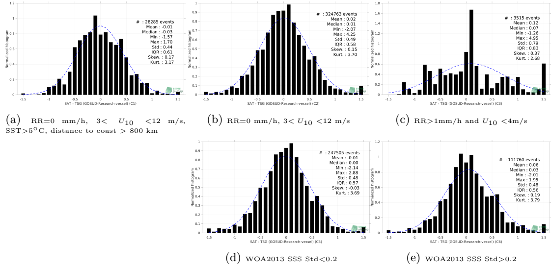
Figure 13: Normalized histogram of \Delta SSS (SMAP SSS L2 v5 (RSS) - TSG (GOSUD-Research-vessel)) for 5 different subdatasets corresponding to: RR=0 mm/h, 3 < U_{10} < 12 m/s, SST > 5°C, distance to coast > 800 km (a), RR=0 mm/h, 3 < U_{10} < 12 m/s (b), RR > 1mm/h and U_{10} < 4 m/s (c), WOA2013 SSS Std < 0.2 (d), WOA2013 SSS Std > 0.2 (e).
