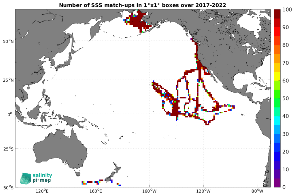
Figure 4: Number of SSS match-ups between Saildrone SSS and the SMAP SSS L2 v5 (RSS) SSS product for the Pacific Ocean Pi-MEP region over 1^\circ \times 1^\circ boxes and for the full satellite product period.
