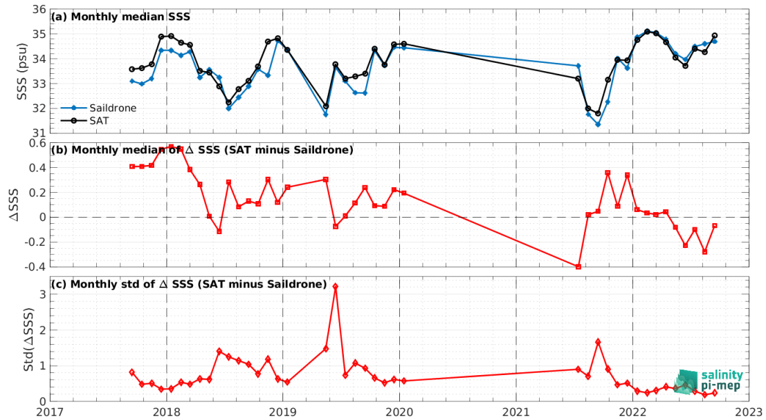
Figure 7: Time series of the monthly median SSS (top), median of \Delta\text{SSS} (Satellite - Sairdron) and Std of \Delta\text{SSS} (Satellite - Sairdron) over the Pacific Ocean Pi-MEP region considering all match-ups collected by the Pi-MEP.
