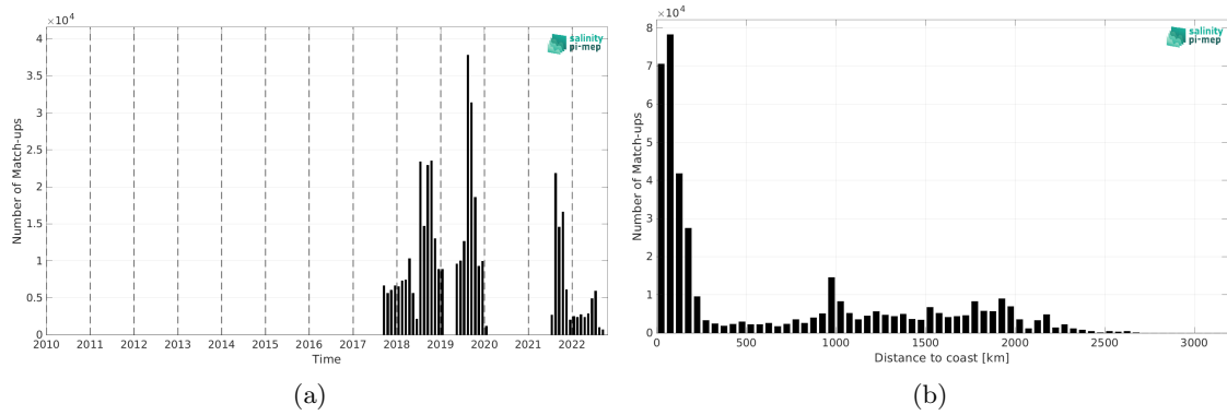
Figure 1: Number of match-ups between Sairdrone and SMAP SSS L2 v5 (RSS) SSS as a function of time (a) and as function of the distance to coast (b) over the Pacific Ocean Pi-MEP region and for the full satellite product period.
