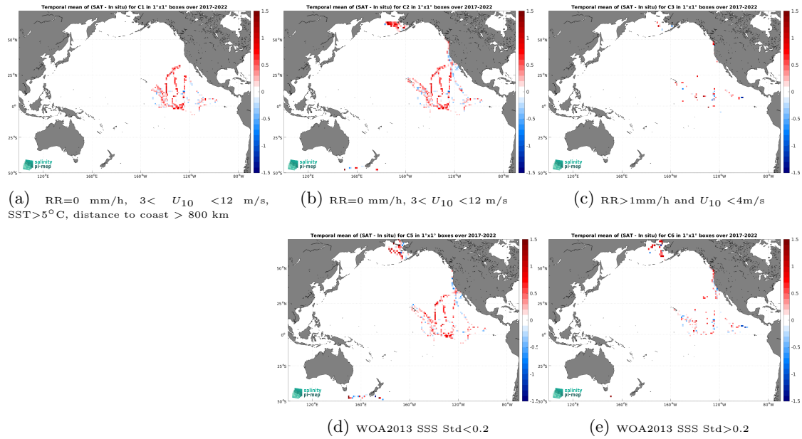
Figure 12: Temporal mean gridded over spatial boxes of size 1^\circ \times 1^\circ of \Delta SSS (SMAP SSS L2 v5 (RSS) - Saifdrone) for 5 different subdatasets corresponding to:RR=0 mm/h, 3 < U_{10} < 12 m/s, SST >5^\circ C, distance to coast > 800 km (a), RR=0 mm/h, 3 < U_{10} < 12 m/s (b), RR >1 mm/h and U_{10} < 4 m/s (c), WOA2013 SSS Std <0.2 (d), WOA2013 SSS Std >0.2 (e).
