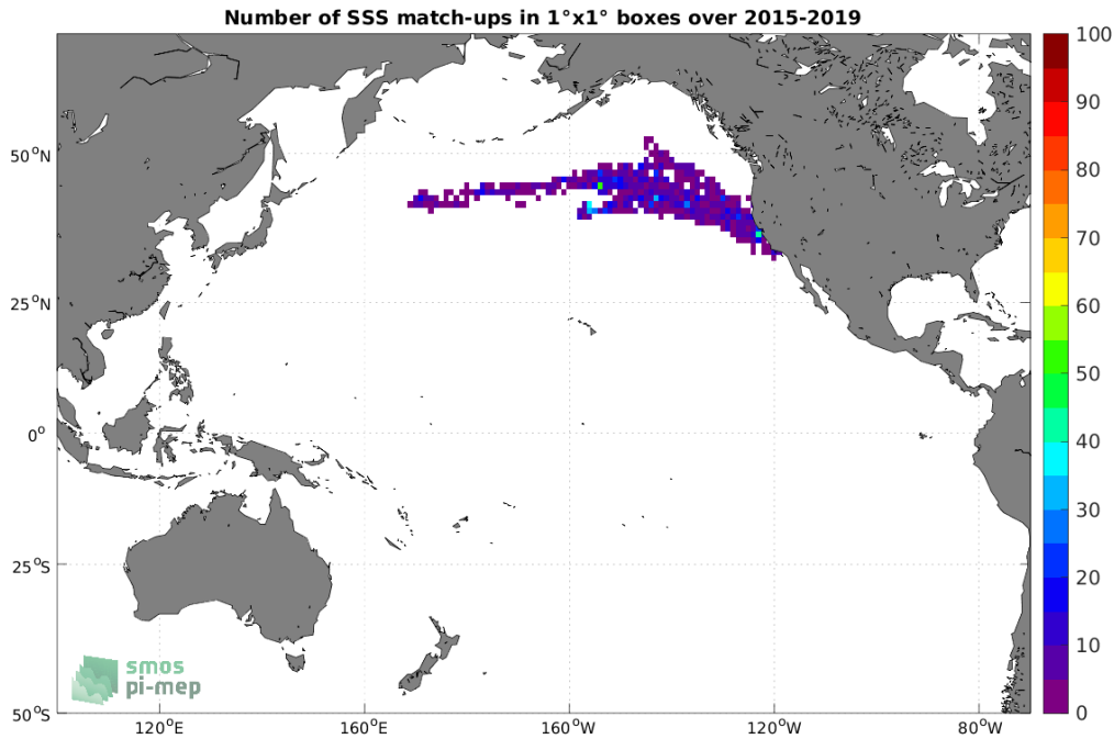
Figure 4: Number of SSS match-ups between Marine mammals SSS and the SMAP SSS L2 v5 (RSS) SSS product for the Pacific Ocean Pi-MEP region over 1°×1° boxes and for the full satellite product period.
