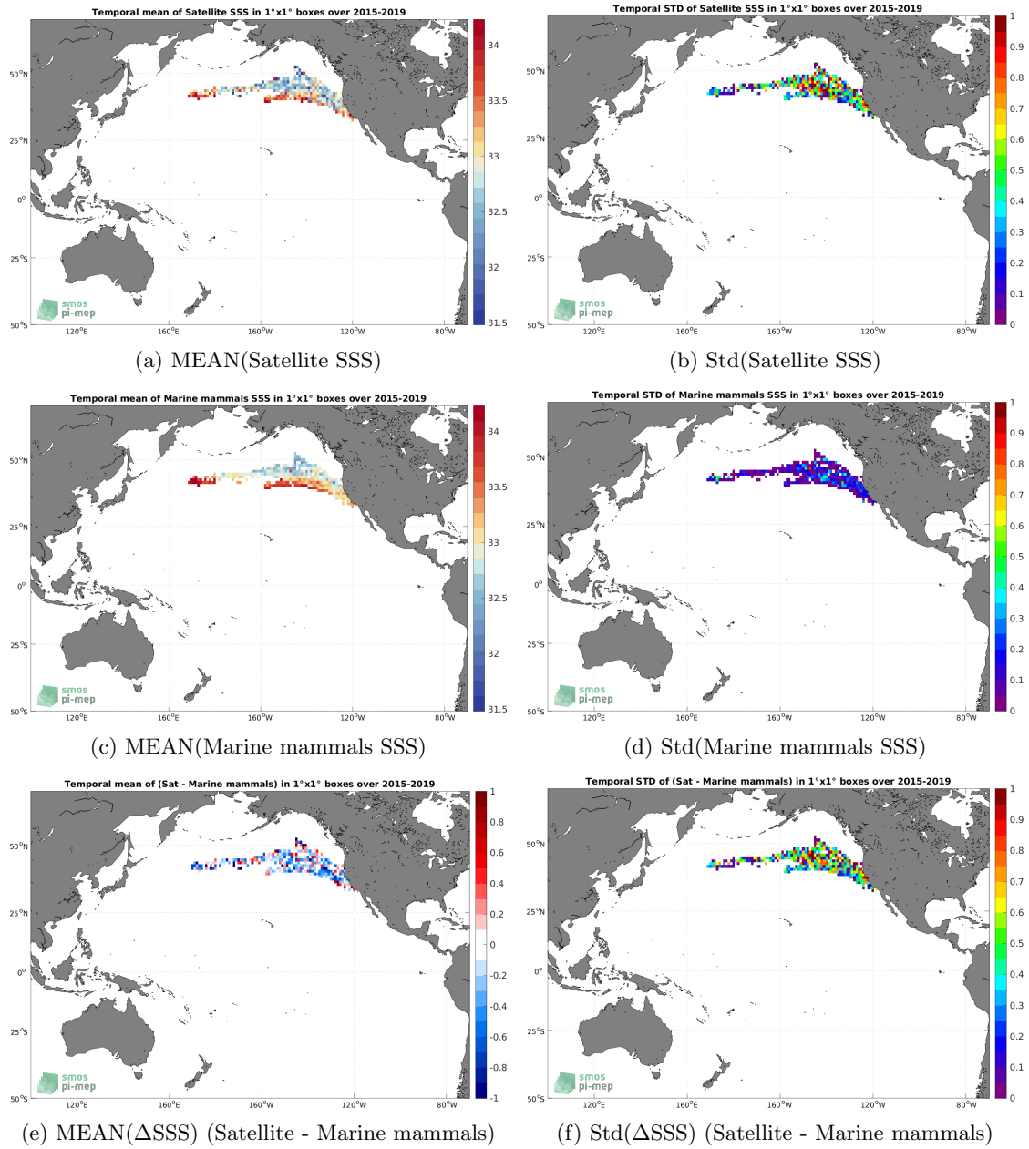
Figure 6: Temporal mean (left) and Std (right) of SSS from SMAP SSS L2 v5 (RSS) (top), Marine mammals (middle), and of \Delta SSS (Satellite - Marine mammals). Only match-up pairs are used to generate these maps.
