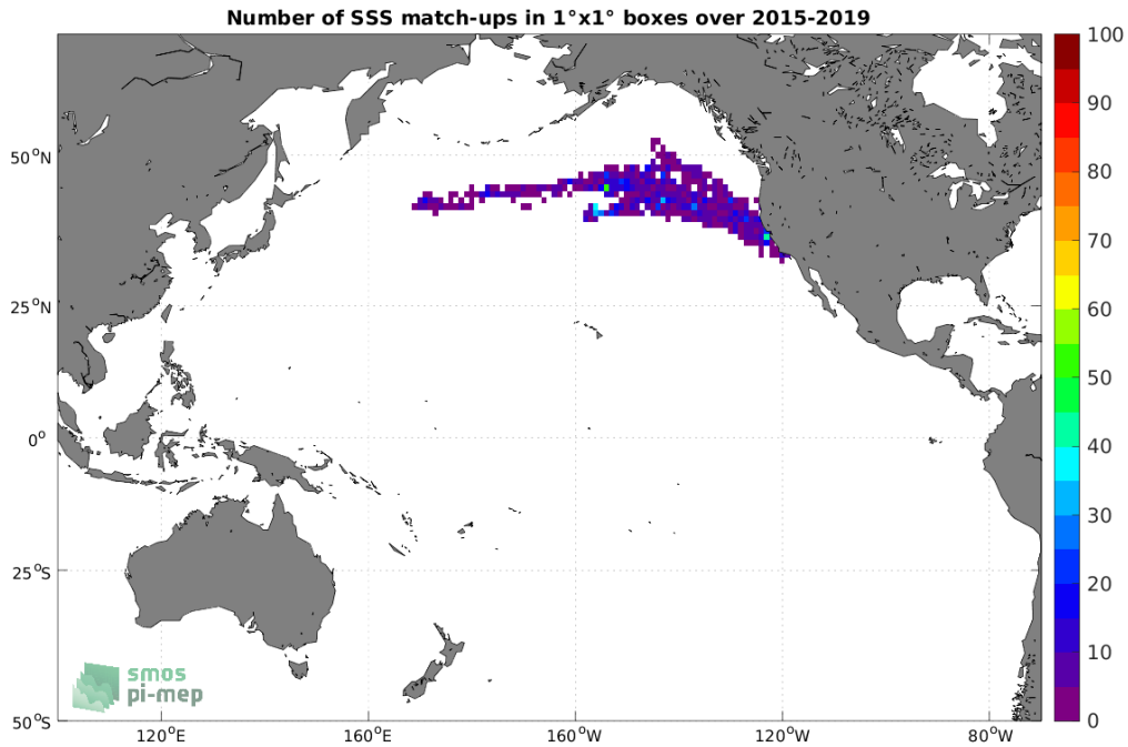
Figure 4: Number of SSS match-ups between Marine mammals SSS and the SMAP SSS L2 v5 (RSS) SSS product for the Pacific Ocean Pi-MEP region over 1^\circ \times 1^\circ boxes and for the full satellite product period.
