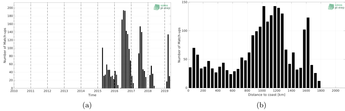
Figure 1: Number of match-ups between Marine mammals and SMAP SSS L2 v5 (RSS) SSS as a function of time (a) and as function of the distance to coast (b) over the Pacific Ocean Pi-MEP region and for the full satellite product period.
