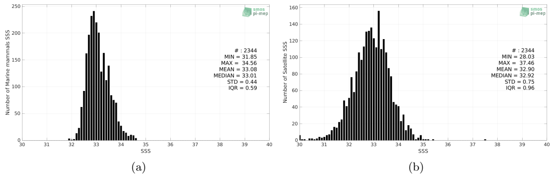
Figure 2: Histograms of SSS from Marine mammals (a) and SMAP SSS L2 v5 (RSS) (b) considering all match-up pairs per bins of 0.1 over the Pacific Ocean Pi-MEP region and for the full satellite product period.
