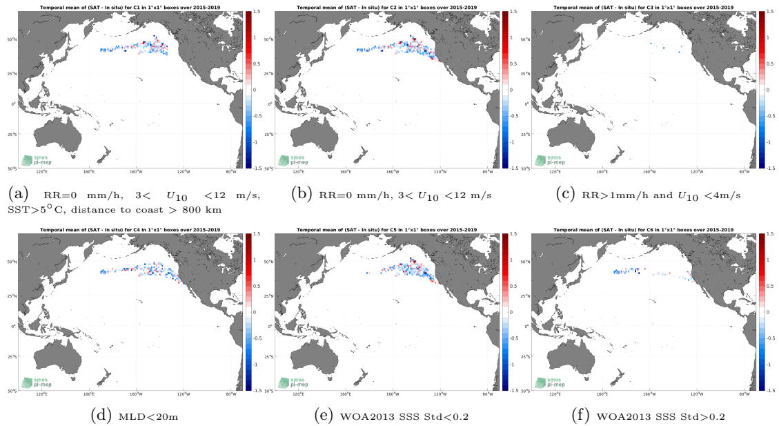
Figure 12: Temporal mean gridded over spatial boxes of size 1^\circ \times 1^\circ of \Delta SSS (SMAP SSS L2 v5 (RSS) - Marine mammals) for 6 different subdatasets corresponding to:RR=0 mm/h, 3 < U_{10} < 12 m/s, SST > 5^\circ\text{C} , distance to coast > 800 km (a), RR=0 mm/h, 3 < U_{10} < 12 m/s (b), RR > 1 mm/h and U_{10} < 4 m/s (c),MLD < 20 m (d),WOA2013 SSS Std < 0.2 (e),WOA2013 SSS Std > 0.2 (f).
