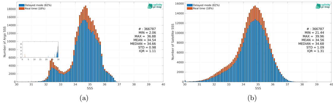
Figure 2: Histograms of SSS from Argo (a) and SMAP SSS L2 v5 (RSS) (b) considering all match-up pairs per bins of 0.1 over the Pacific Ocean Pi-MEP region and for the full satellite product period.
