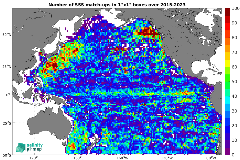
Figure 4: Number of SSS match-ups between Argo SSS and the SMAP SSS L2 v5 (RSS) SSS product for the Pacific Ocean Pi-MEP region over 1^\circ \times 1^\circ boxes and for the full satellite product period.
