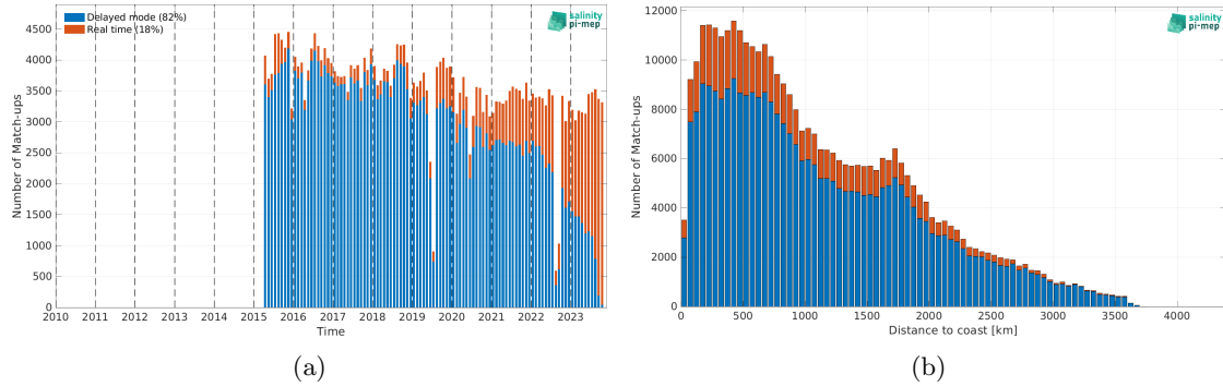
Figure 1: Number of match-ups between Argo and SMAP SSS L2 v5 (RSS) SSS as a function of time (a) and as function of the distance to coast (b) over the Pacific Ocean Pi-MEP region and for the full satellite product period.
