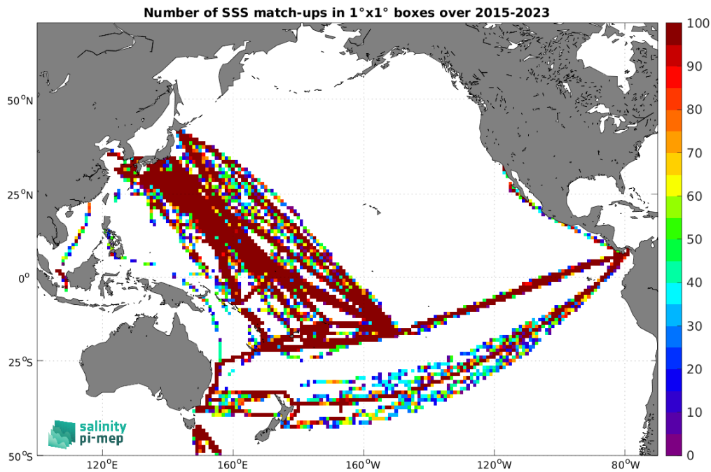
Figure 5: Number of SSS match-ups between TSG (LEGOS-DM) SSS and the SMAP SSS L2 v5.3 (RSS) SSS product for the Pacific Ocean Pi-MEP region over 1^\circ \times 1^\circ boxes and for the full satellite product period.
