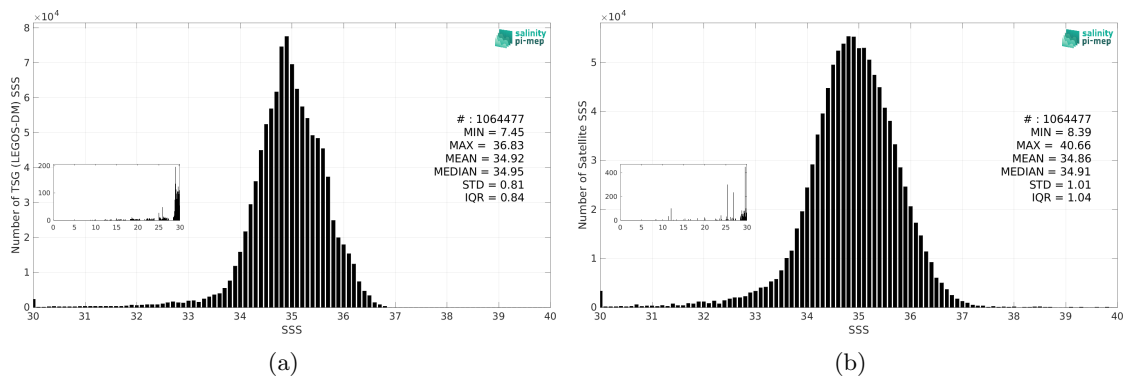
Figure 3: Histograms of SSS from TSG (LEGOS-DM) (a) and SMAP SSS L2 v5.3 (RSS) (b) considering all match-up pairs per bins of 0.1 over the Pacific Ocean Pi-MEP region and for the full satellite product period.
