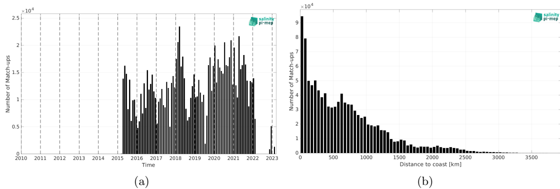
Figure 2: Number of match-ups between TSG (LEGOS-DM) and SMAP SSS L2 v5.3 (RSS) SSS as a function of time (a) and as function of the distance to coast (b) over the Pacific Ocean Pi-MEP region and for the full satellite product period.
