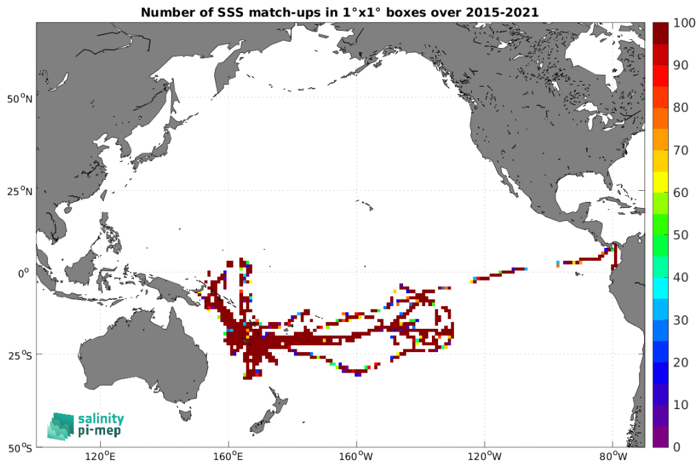
Figure 5: Number of SSS match-ups between TSG (GOSUD-Research-vessel) SSS and the SMAP SSS L2 v5.3 (RSS) SSS product for the Pacific Ocean Pi-MEP region over 1^\circ \times 1^\circ boxes and for the full satellite product period.
