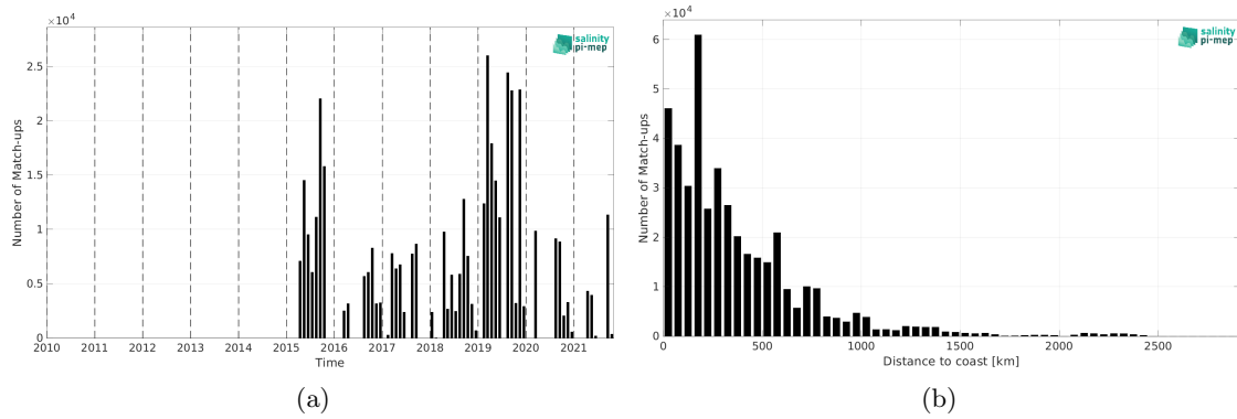
Figure 2: Number of match-ups between TSG (GOSUD-Research-vessel) and SMAP SSS L2 v5.3 (RSS) SSS as a function of time (a) and as function of the distance to coast (b) over the Pacific Ocean Pi-MEP region and for the full satellite product period.
