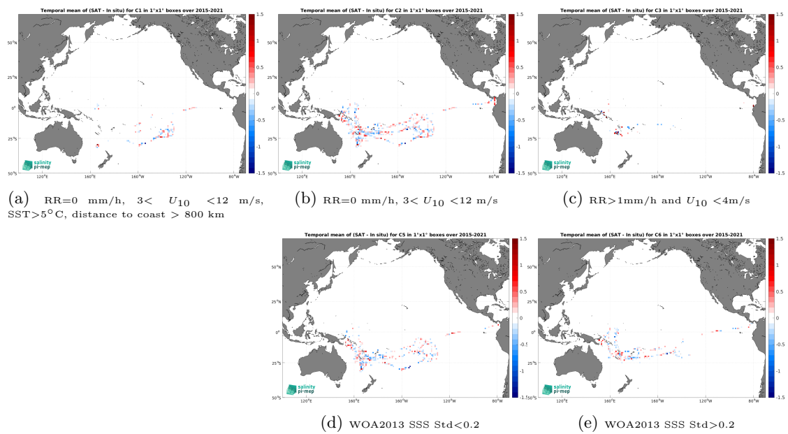
Figure 14: Temporal mean gridded over spatial boxes of size 1^\circ \times 1^\circ of \Delta SSS (SMAP SSS L2 v5.3 (RSS) - TSG (GOSUD-Research-vessel)) for 5 different subdatasets corresponding to:RR=0 mm/h, 3 < U_{10} < 12 m/s, SST>5°C, distance to coast > 800 km (a), RR=0 mm/h, 3 < U_{10} < 12 m/s (b), RR>1mm/h and U_{10} < 4 m/s (c), WOA2013 SSS Std<0.2 (d), WOA2013 SSS Std>0.2 (e).
