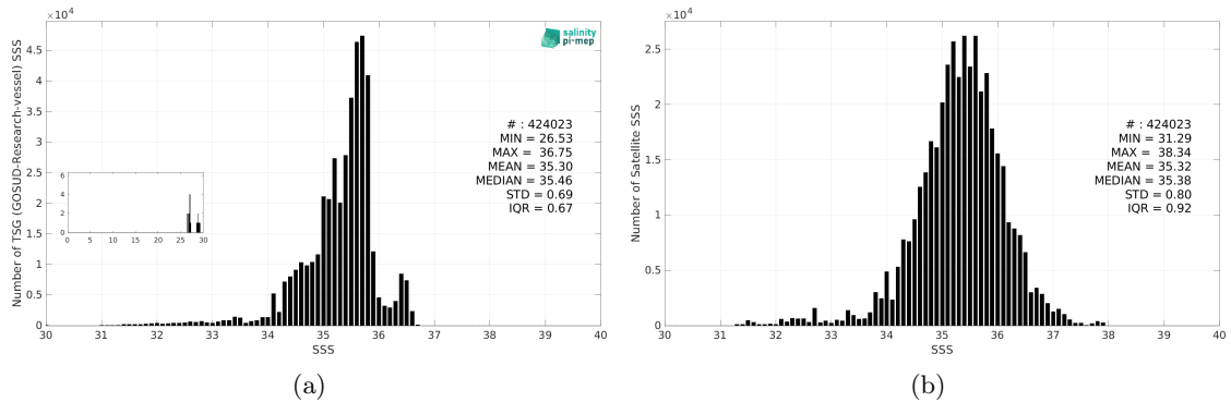
Figure 3: Histograms of SSS from TSG (GOSUD-Research-vessel) (a) and SMAP SSS L2 v5.3 (RSS) (b) considering all match-up pairs per bins of 0.1 over the Pacific Ocean Pi-MEP region and for the full satellite product period.
