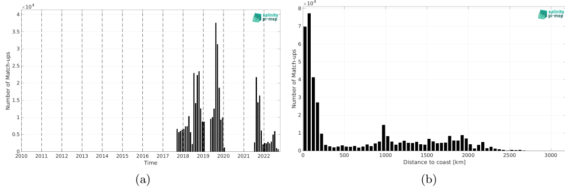
Figure 2: Number of match-ups between Saildrone and SMAP SSS L2 v5.3 (RSS) SSS as a function of time (a) and as function of the distance to coast (b) over the Pacific Ocean Pi-MEP region and for the full satellite product period.
