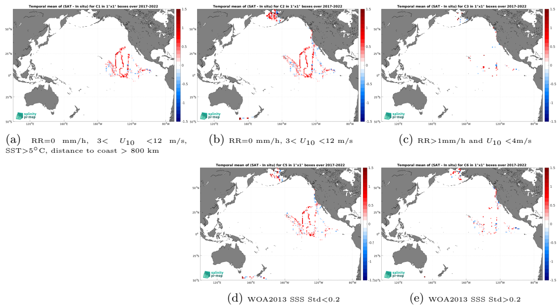
Figure 14: Temporal mean gridded over spatial boxes of size 1^\circ \times 1^\circ of \Delta SSS (SMAP SSS L2 v5.3 (RSS) - Saifdrone) for 5 different subdatasets corresponding to: RR=0 mm/h, 3 < U_{10} < 12 m/s, SST > 5°C, distance to coast > 800 km (a), RR=0 mm/h, 3 < U_{10} < 12 m/s (b), RR > 1mm/h and U_{10} < 4 m/s (c), WOA2013 SSS Std < 0.2 (d), WOA2013 SSS Std > 0.2 (e).
