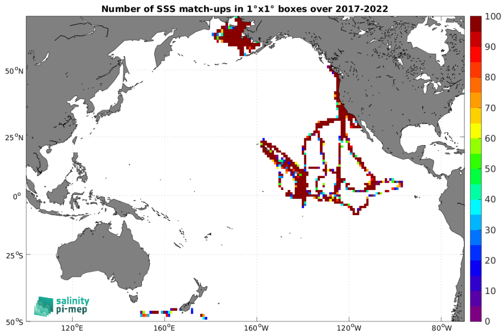
Figure 5: Number of SSS match-ups between Saildrone SSS and the SMAP SSS L2 v5.3 (RSS) SSS product for the Pacific Ocean Pi-MEP region over 1^\circ \times 1^\circ boxes and for the full satellite product period.
