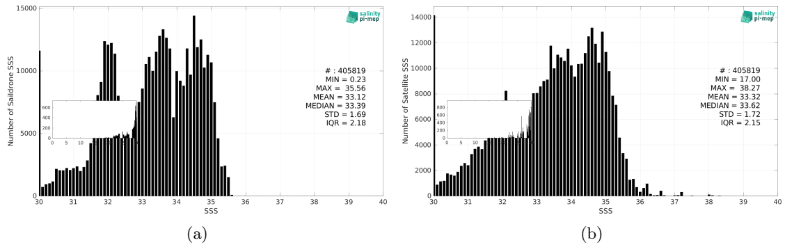
Figure 3: Histograms of SSS from Saildrone (a) and SMAP SSS L2 v5.3 (RSS) (b) considering all match-up pairs per bins of 0.1 over the Pacific Ocean Pi-MEP region and for the full satellite product period.
