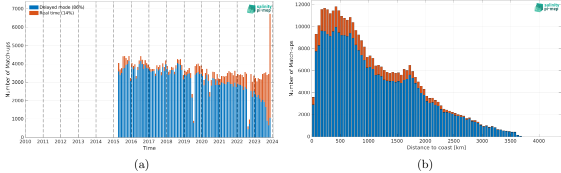
Figure 2: Number of match-ups between Argo and SMAP SSS L2 v5.3 (RSS) SSS as a function of time (a) and as function of the distance to coast (b) over the Pacific Ocean Pi-MEP region and for the full satellite product period.
