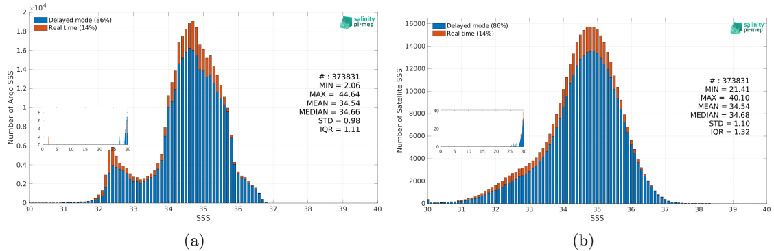
Figure 3: Histograms of SSS from Argo (a) and SMAP SSS L2 v5.3 (RSS) (b) considering all match-up pairs per bins of 0.1 over the Pacific Ocean Pi-MEP region and for the full satellite product period.
