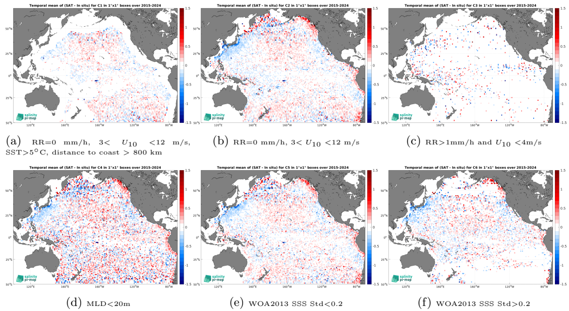
Figure 14: Temporal mean gridded over spatial boxes of size 1^\circ \times 1^\circ of \Delta SSS (SMAP SSS L2 v5.3 (RSS) - Argo) for 6 different subdatasets corresponding to: RR=0 mm/h, 3 < U_{10} < 12 m/s, SST > 5°C, distance to coast > 800 km (a), RR=0 mm/h, 3 < U_{10} < 12 m/s (b), RR > 1mm/h and U_{10} < 4 m/s (c), MLD < 20m (d), WOA2013 SSS Std < 0.2 (e), WOA2013 SSS Std > 0.2 (f).
