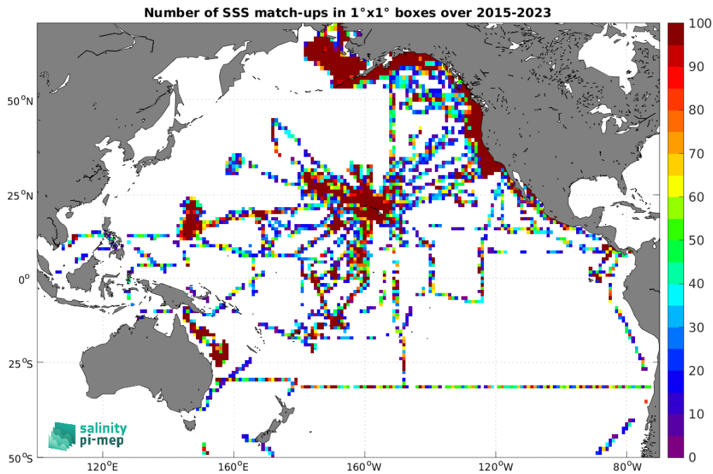
Figure 5: Number of SSS match-ups between TSG (SAMOS) SSS and the SMAP SSS L2 v5.3 - 40 km (RSS) SSS product for the Pacific Ocean Pi-MEP region over 1^\circ \times 1^\circ boxes and for the full satellite product period.
