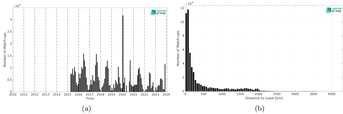
Figure 2: Number of match-ups between TSG (SAMOS) and SMAP SSS L2 v5.3 - 40 km (RSS) SSS as a function of time (a) and as function of the distance to coast (b) over the Pacific Ocean Pi-MEP region and for the full satellite product period.
