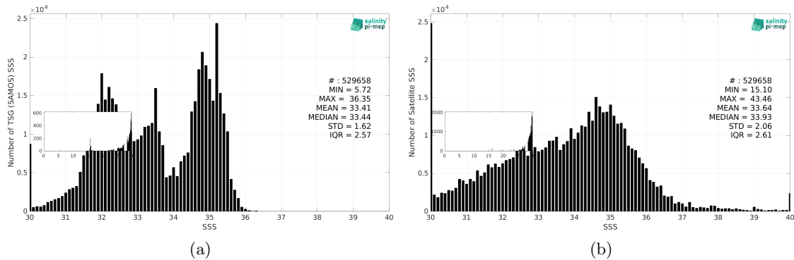
Figure 3: Histograms of SSS from TSG (SAMOS) (a) and SMAP SSS L2 v5.3 - 40 km (RSS) (b) considering all match-up pairs per bins of 0.1 over the Pacific Ocean Pi-MEP region and for the full satellite product period.
