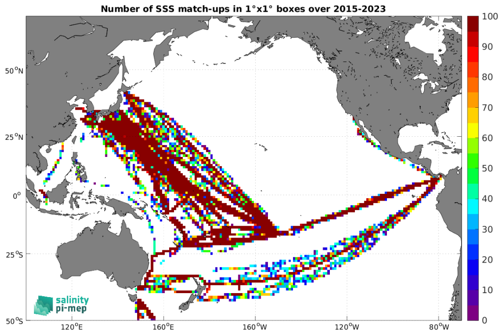
Figure 5: Number of SSS match-ups between TSG (LEGOS-DM) SSS and the SMAP SSS L2 v5.3 - 40 km (RSS) SSS product for the Pacific Ocean Pi-MEP region over 1^\circ \times 1^\circ boxes and for the full satellite product period.
