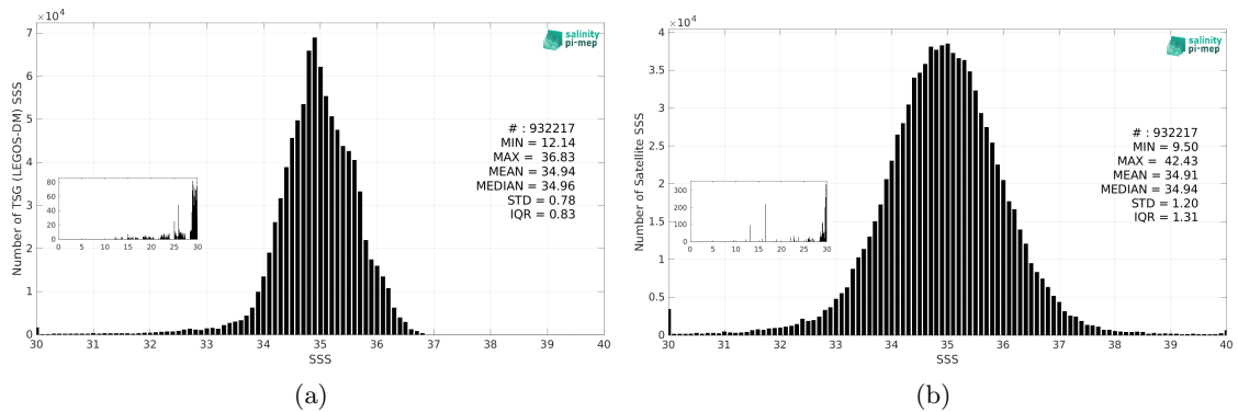
Figure 3: Histograms of SSS from TSG (LEGOS-DM) (a) and SMAP SSS L2 v5.3 - 40 km (RSS) (b) considering all match-up pairs per bins of 0.1 over the Pacific Ocean Pi-MEP region and for the full satellite product period.
