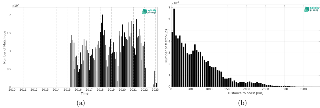
Figure 2: Number of match-ups between TSG (LEGOS-DM) and SMAP SSS L2 v5.3 - 40 km (RSS) SSS as a function of time (a) and as function of the distance to coast (b) over the Pacific Ocean Pi-MEP region and for the full satellite product period.
