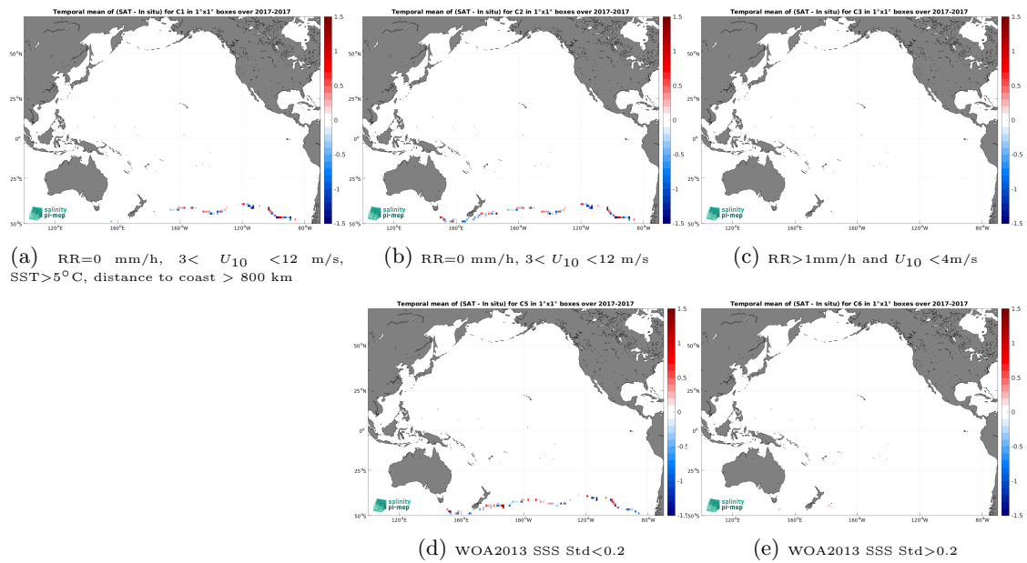
Figure 14: Temporal mean gridded over spatial boxes of size 1^\circ \times 1^\circ of \Delta SSS (SMAP SSS L2 v5.3 - 40 km (RSS) - TSG (GOSUD-Sailing-ship)) for 5 different subdatasets corresponding to:RR=0 mm/h, 3 < U_{10} < 12 m/s, SST > 5°C, distance to coast > 800 km (a), RR=0 mm/h, 3 < U_{10} < 12 m/s (b), RR > 1mm/h and U_{10} < 4 m/s (c), WOA2013 SSS Std < 0.2 (d), WOA2013 SSS Std > 0.2 (e).
