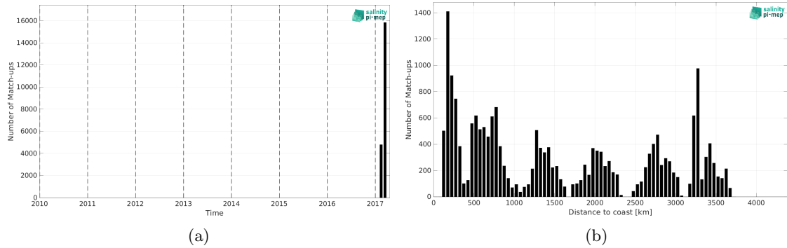
Figure 2: Number of match-ups between TSG (GOSUD-Sailing-ship) and SMAP SSS L2 v5.3 - 40 km (RSS) SSS as a function of time (a) and as function of the distance to coast (b) over the Pacific Ocean Pi-MEP region and for the full satellite product period.
