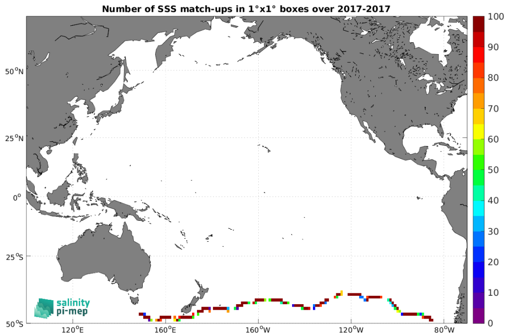
Figure 5: Number of SSS match-ups between TSG (GOSUD-Sailing-ship) SSS and the SMAP SSS L2 v5.3 - 40 km (RSS) SSS product for the Pacific Ocean Pi-MEP region over 1^\circ \times 1^\circ boxes and for the full satellite product period.
