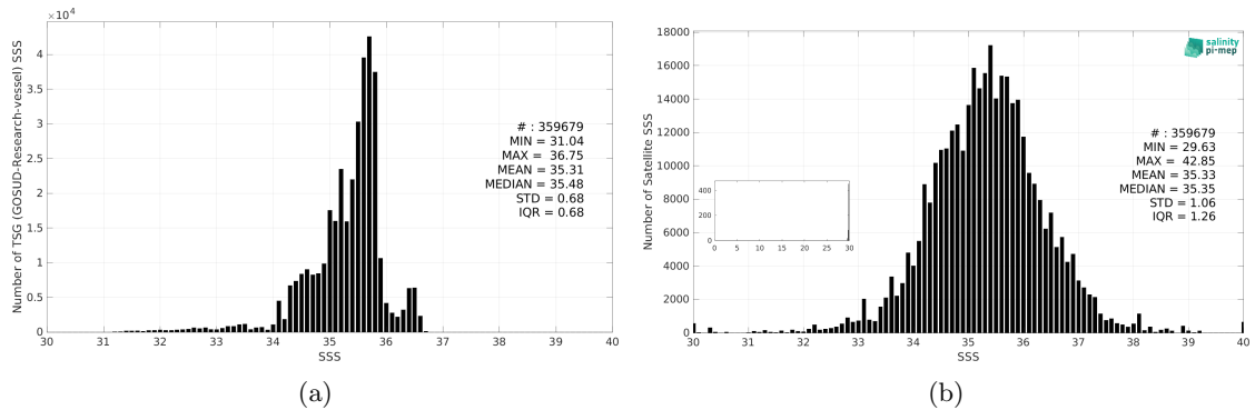
Figure 3: Histograms of SSS from TSG (GOSUD-Research-vessel) (a) and SMAP SSS L2 v5.3 - 40 km (RSS) (b) considering all match-up pairs per bins of 0.1 over the Pacific Ocean Pi-MEP region and for the full satellite product period.
