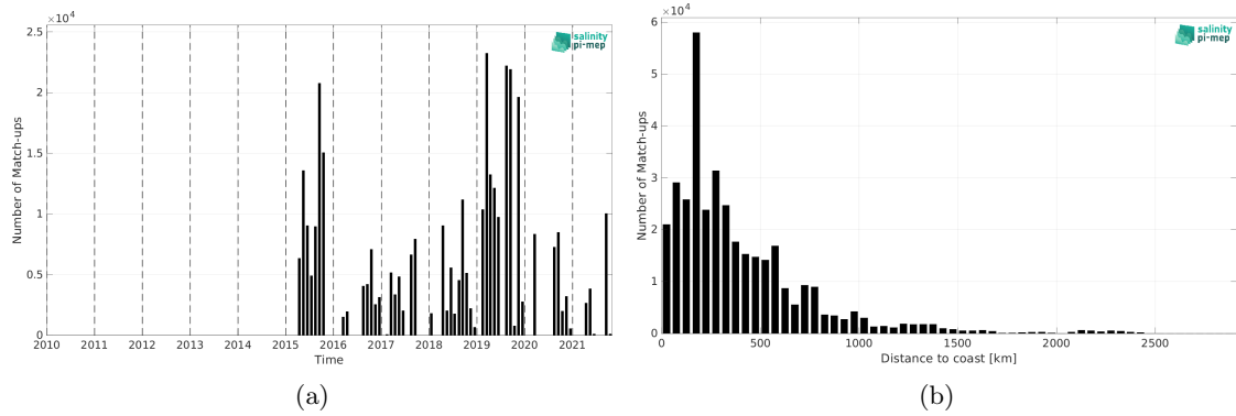
Figure 2: Number of match-ups between TSG (GOSUD-Research-vessel) and SMAP SSS L2 v5.3 - 40 km (RSS) SSS as a function of time (a) and as function of the distance to coast (b) over the Pacific Ocean Pi-MEP region and for the full satellite product period.
