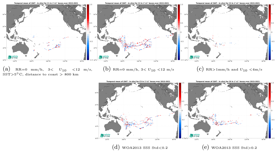
Figure 14: Temporal mean gridded over spatial boxes of size 1^\circ \times 1^\circ of \Delta SSS (SMAP SSS L2 v5.3 - 40 km (RSS) - TSG (GOSUD-Research-vessel)) for 5 different subdatasets corresponding to: RR=0 mm/h, 3 < U_{10} < 12 m/s, SST > 5^\circ\text{C} , distance to coast > 800 km (a), RR=0 mm/h, 3 < U_{10} < 12 m/s (b), RR > 1 mm/h and U_{10} < 4 m/s (c), WOA2013 SSS Std < 0.2 (d), WOA2013 SSS Std > 0.2 (e).
