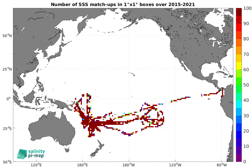
Figure 5: Number of SSS match-ups between TSG (GOSUD-Research-vessel) SSS and the SMAP SSS L2 v5.3 - 40 km (RSS) SSS product for the Pacific Ocean Pi-MEP region over 1^\circ \times 1^\circ boxes and for the full satellite product period.
