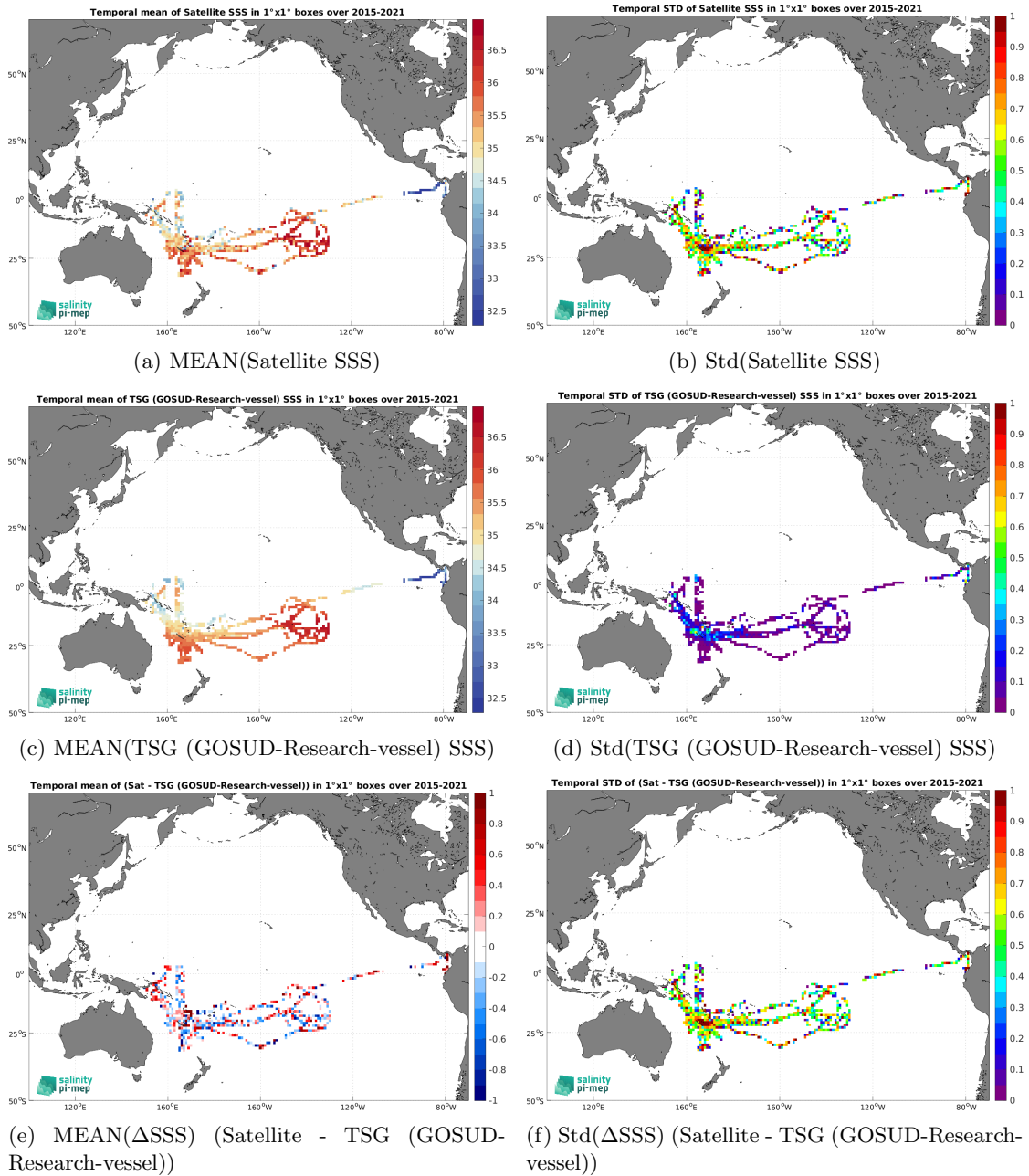
Figure 7: Temporal mean (left) and Std (right) of SSS from SMAP SSS L2 v5.3 - 40 km (RSS) (top), TSG (GOSUD-Research-vessel) (middle), and of \Delta SSS (Satellite - TSG (GOSUD-Research-vessel)). Only match-up pairs are used to generate these maps.
