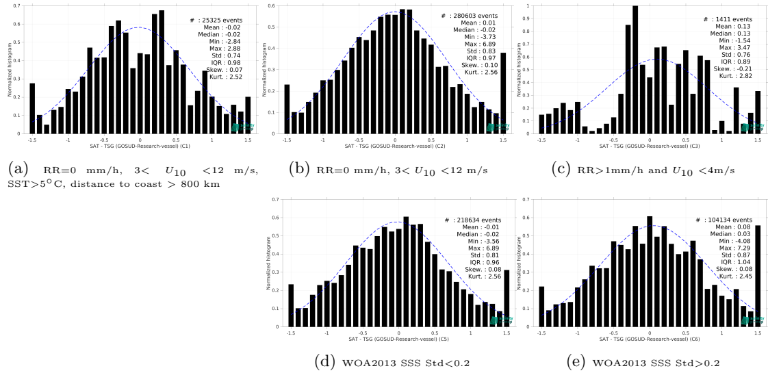
Figure 15: Normalized histogram of \Delta SSS (SMAP SSS L2 v5.3 - 40 km (RSS) - TSG (GOSUD-Research-vessel)) for 5 different subdatasets corresponding to: RR=0 mm/h, 3 < U_{10} < 12 m/s, SST > 5°C, distance to coast > 800 km (a), RR=0 mm/h, 3 < U_{10} < 12 m/s (b), RR > 1mm/h and U_{10} < 4 m/s (c), WOA2013 SSS Std < 0.2 (d), WOA2013 SSS Std > 0.2 (e).
