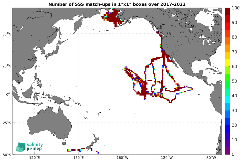
Figure 5: Number of SSS match-ups between Saildrone SSS and the SMAP SSS L2 v5.3 - 40 km (RSS) SSS product for the Pacific Ocean Pi-MEP region over 1^\circ \times 1^\circ boxes and for the full satellite product period.
