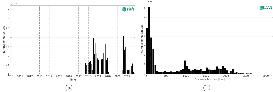
Figure 2: Number of match-ups between Sailldrone and SMAP SSS L2 v5.3 - 40 km (RSS) SSS as a function of time (a) and as function of the distance to coast (b) over the Pacific Ocean Pi-MEP region and for the full satellite product period.
