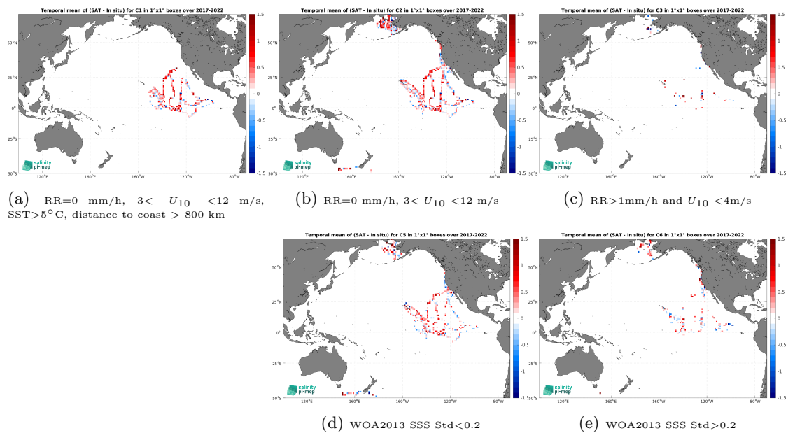
Figure 14: Temporal mean gridded over spatial boxes of size 1^\circ \times 1^\circ of \Delta SSS (SMAP SSS L2 v5.3 - 40 km (RSS) - Saildrone) for 5 different subdatasets corresponding to: RR=0 mm/h, 3 < U_{10} < 12 m/s, SST > 5^\circ\text{C} , distance to coast > 800 km (a), RR=0 mm/h, 3 < U_{10} < 12 m/s (b), RR > 1 mm/h and U_{10} < 4 m/s (c), WOA2013 SSS Std < 0.2 (d), WOA2013 SSS Std > 0.2 (e).
