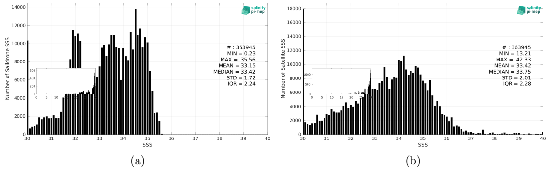
Figure 3: Histograms of SSS from Sailldrone (a) and SMAP SSS L2 v5.3 - 40 km (RSS) (b) considering all match-up pairs per bins of 0.1 over the Pacific Ocean Pi-MEP region and for the full satellite product period.
