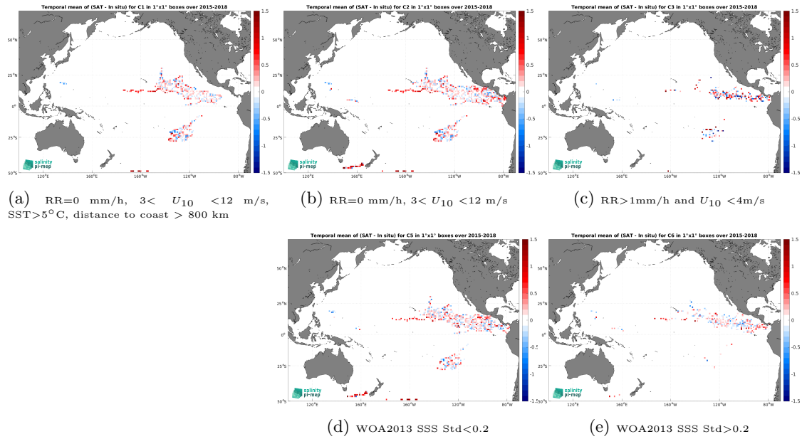
Figure 13: Temporal mean gridded over spatial boxes of size 1^\circ \times 1^\circ of \Delta SSS (SMAP SSS L2 v5.3 - 40 km (RSS) - Surface drifters) for 5 different subdatasets corresponding to:RR=0 mm/h, 3 < U_{10} < 12 m/s, SST >5^\circ C, distance to coast > 800 km (a), RR=0 mm/h, 3 < U_{10} < 12 m/s (b), RR >1 mm/h and U_{10} < 4 m/s (c), WOA2013 SSS Std <0.2 (d), WOA2013 SSS Std >0.2 (e).
