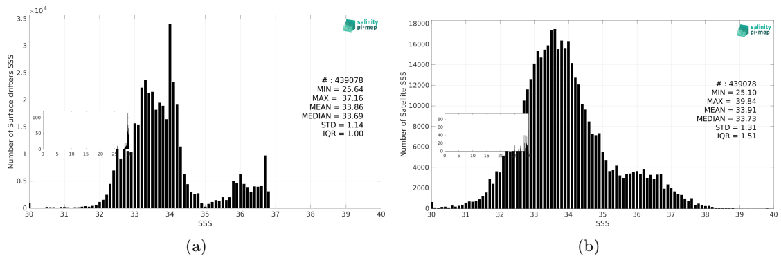
Figure 3: Histograms of SSS from Surface drifters (a) and SMAP SSS L2 v5.3 - 40 km (RSS) (b) considering all match-up pairs per bins of 0.1 over the Pacific Ocean Pi-MEP region and for the full satellite product period.
