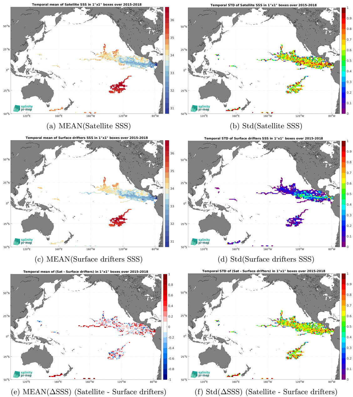
Figure 6: Temporal mean (left) and Std (right) of SSS from SMAP SSS L2 v5.3 - 40 km (RSS) (top), Surface drifters (middle), and of \Delta SSS (Satellite - Surface drifters). Only match-up pairs are used to generate these maps.
