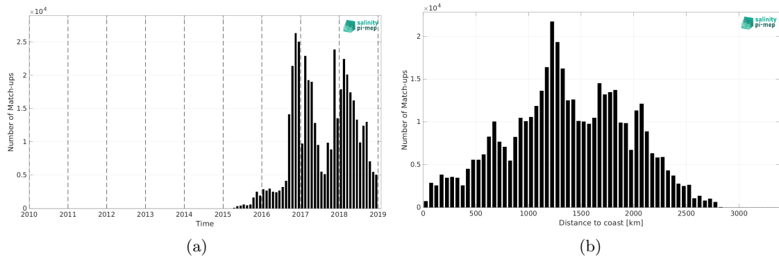
Figure 2: Number of match-ups between Surface drifters and SMAP SSS L2 v5.3 - 40 km (RSS) SSS as a function of time (a) and as function of the distance to coast (b) over the Pacific Ocean Pi-MEP region and for the full satellite product period.
