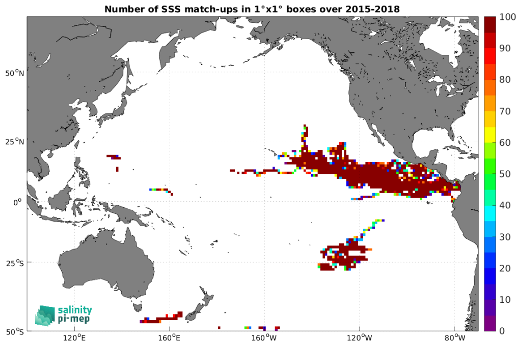
Figure 4: Number of SSS match-ups between Surface drifters SSS and the SMAP SSS L2 v5.3 - 40 km (RSS) SSS product for the Pacific Ocean Pi-MEP region over 1^\circ \times 1^\circ boxes and for the full satellite product period.
