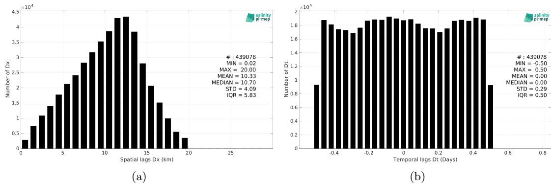
Figure 5: Histograms of the spatial (a) and temporal (b) lags between the location/time of the Surface drifters measurement and the date of the corresponding SMAP SSS L2 v5.3 - 40 km (RSS) SSS pixel.
