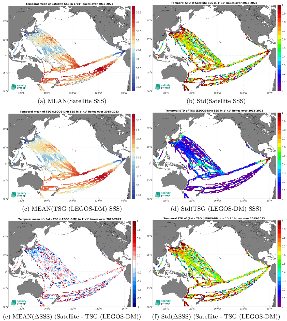
Figure 6: Temporal mean (left) and Std (right) of SSS from SMAP SSS L2 v5 - 40 km (RSS) (top), TSG (LEGOS-DM) (middle), and of \Delta SSS (Satellite - TSG (LEGOS-DM)). Only match-up pairs are used to generate these maps.
