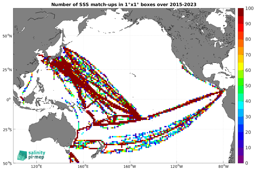
Figure 4: Number of SSS match-ups between TSG (LEGOS-DM) SSS and the SMAP SSS L2 v5 - 40 km (RSS) SSS product for the Pacific Ocean Pi-MEP region over 1^\circ \times 1^\circ boxes and for the full satellite product period.
