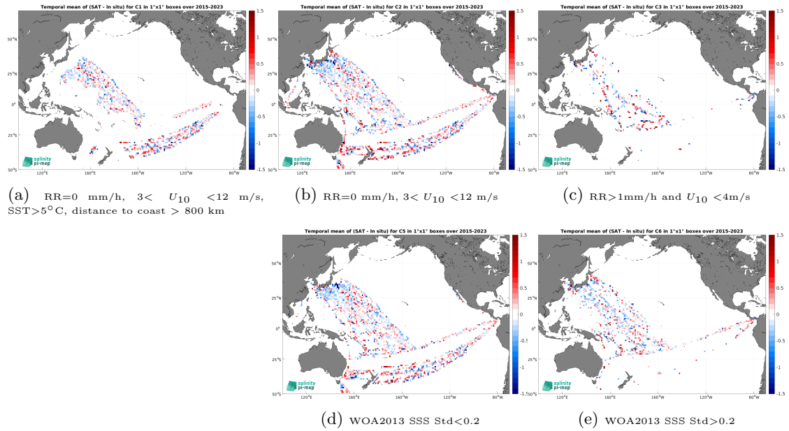
Figure 12: Temporal mean gridded over spatial boxes of size 1^\circ \times 1^\circ of \Delta SSS (SMAP SSS L2 v5 - 40 km (RSS) - TSG (LEGOS-DM)) for 5 different subdatasets corresponding to:RR=0 mm/h, 3 < U_{10} < 12 m/s, SST >5^\circ C, distance to coast > 800 km (a), RR=0 mm/h, 3 < U_{10} < 12 m/s (b), RR >1 mm/h and U_{10} < 4 m/s (c), WOA2013 SSS Std <0.2 (d), WOA2013 SSS Std >0.2 (e).
