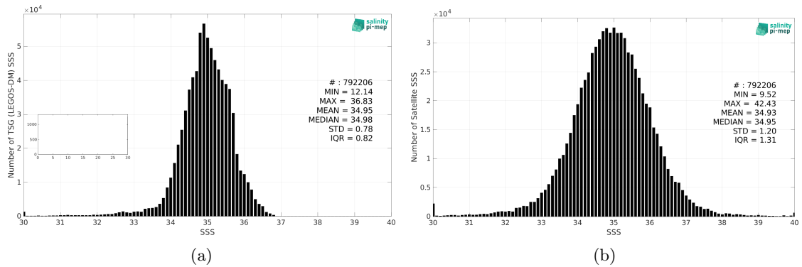
Figure 2: Histograms of SSS from TSG (LEGOS-DM) (a) and SMAP SSS L2 v5 - 40 km (RSS) (b) considering all match-up pairs per bins of 0.1 over the Pacific Ocean Pi-MEP region and for the full satellite product period.
