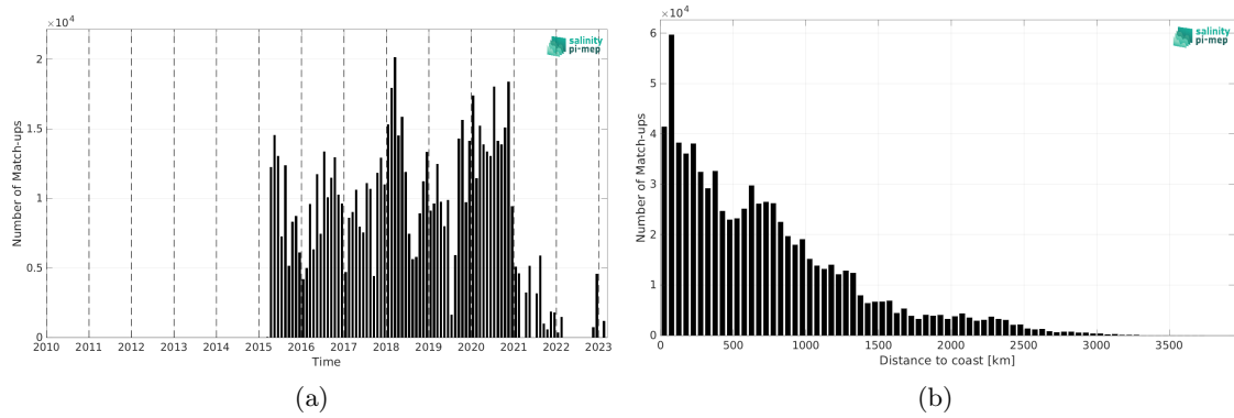
Figure 1: Number of match-ups between TSG (LEGOS-DM) and SMAP SSS L2 v5 - 40 km (RSS) SSS as a function of time (a) and as function of the distance to coast (b) over the Pacific Ocean Pi-MEP region and for the full satellite product period.
