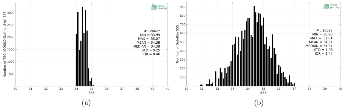
Figure 2: Histograms of SSS from TSG (GOSUD-Sailing-ship) (a) and SMAP SSS L2 v5 - 40 km (RSS) (b) considering all match-up pairs per bins of 0.1 over the Pacific Ocean Pi-MEP region and for the full satellite product period.
