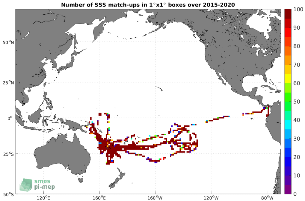
Figure 4: Number of SSS match-ups between TSG (GOSUD-Research-vessel) SSS and the SMAP SSS L2 v5 - 40 km (RSS) SSS product for the Pacific Ocean Pi-MEP region over 1^\circ \times 1^\circ boxes and for the full satellite product period.
