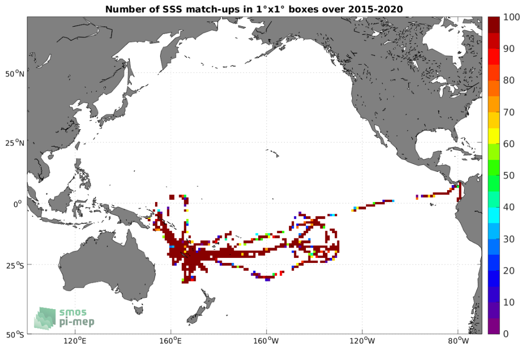
Figure 4: Number of SSS match-ups between TSG (GOSUD-Research-vessel) SSS and the SMAP SSS L2 v5 - 40 km (RSS) SSS product for the Pacific Ocean Pi-MEP region over 1°x1° boxes and for the full satellite product period.
