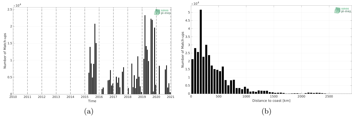
Figure 1: Number of match-ups between TSG (GOSUD-Research-vessel) and SMAP SSS L2 v5 - 40 km (RSS) SSS as a function of time (a) and as function of the distance to coast (b) over the Pacific Ocean Pi-MEP region and for the full satellite product period.
