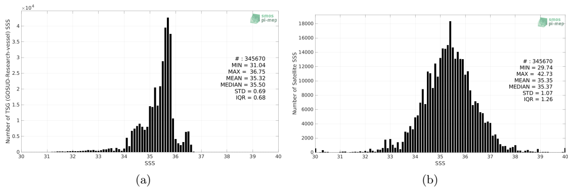
Figure 2: Histograms of SSS from TSG (GOSUD-Research-vessel) (a) and SMAP SSS L2 v5 - 40 km (RSS) (b) considering all match-up pairs per bins of 0.1 over the Pacific Ocean Pi-MEP region and for the full satellite product period.
