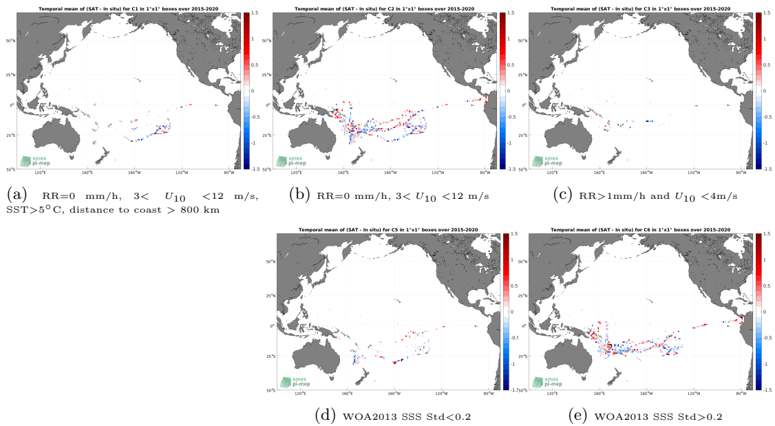
Figure 12: Temporal mean gridded over spatial boxes of size 1^\circ \times 1^\circ of \Delta SSS (SMAP SSS L2 v5 - 40 km (RSS) - TSG (GOSUD-Research-vessel)) for 5 different subdatasets corresponding to: RR=0 mm/h, 3 < U_{10} < 12 m/s, SST > 5°C, distance to coast > 800 km (a), RR=0 mm/h, 3 < U_{10} < 12 m/s (b), RR > 1mm/h and U_{10} < 4 m/s (c), WOA2013 SSS Std < 0.2 (d), WOA2013 SSS Std > 0.2 (e).
