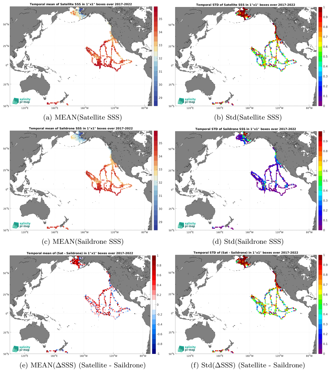
Figure 6: Temporal mean (left) and Std (right) of SSS from SMAP SSS L2 v5 - 40 km (RSS) (top), Saildrone (middle), and of \Delta SSS (Satellite - Saildrone). Only match-up pairs are used to generate these maps.
