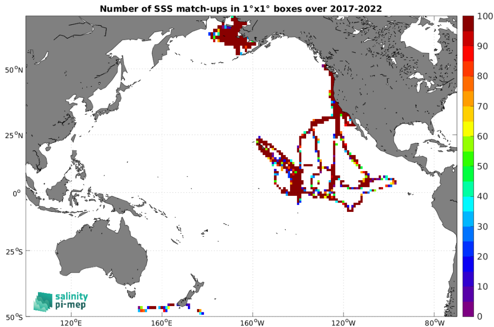
Figure 4: Number of SSS match-ups between Saildrone SSS and the SMAP SSS L2 v5 - 40 km (RSS) SSS product for the Pacific Ocean Pi-MEP region over 1^\circ \times 1^\circ boxes and for the full satellite product period.
