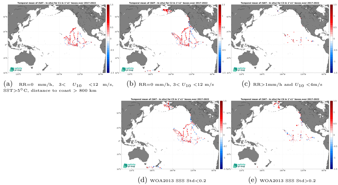
Figure 12: Temporal mean gridded over spatial boxes of size 1^\circ \times 1^\circ of \Delta SSS (SMAP SSS L2 v5 - 40 km (RSS) - Sairdrone) for 5 different subdatasets corresponding to:RR=0 mm/h, 3 < U_{10} < 12 m/s, SST >5^\circ C, distance to coast > 800 km (a), RR=0 mm/h, 3 < U_{10} < 12 m/s (b), RR >1 mm/h and U_{10} < 4 m/s (c), WOA2013 SSS Std <0.2 (d), WOA2013 SSS Std >0.2 (e).
