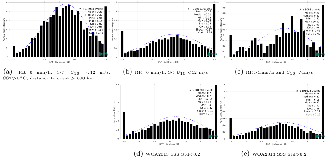
Figure 13: Normalized histogram of \Delta\text{SSS} (SMAP SSS L2 v5 - 40 km (RSS) - Saildrone) for 5 different subdatasets corresponding to: RR=0 mm/h, 3 < U_{10} < 12 m/s, SST>5°C, distance to coast > 800 km (a), RR=0 mm/h, 3 < U_{10} < 12 m/s (b), RR>1mm/h and U_{10} < 4 m/s (c), WOA2013 SSS Std<0.2 (d), WOA2013 SSS Std>0.2 (e).
