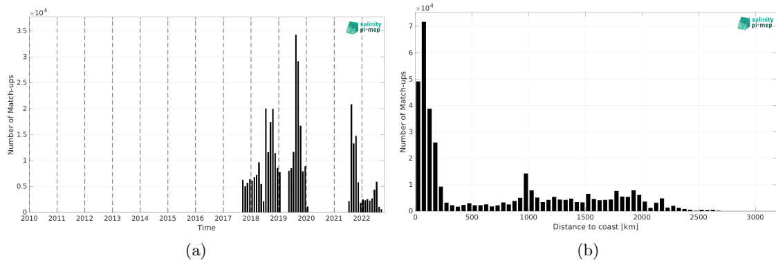
Figure 1: Number of match-ups between Saildrone and SMAP SSS L2 v5 - 40 km (RSS) SSS as a function of time (a) and as function of the distance to coast (b) over the Pacific Ocean Pi-MEP region and for the full satellite product period.
