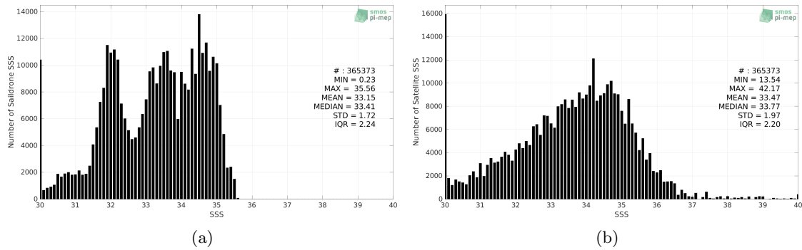
Figure 2: Histograms of SSS from Saifdrone (a) and SMAP SSS L2 v5 - 40 km (RSS) (b) considering all match-up pairs per bins of 0.1 over the Pacific Ocean Pi-MEP region and for the full satellite product period.
