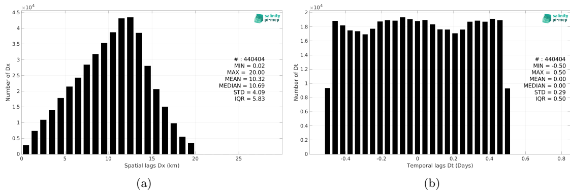
Figure 4: Histograms of the spatial (a) and temporal (b) lags between the location/time of the Surface drifters measurement and the date of the corresponding SMAP SSS L2 v5 - 40 km (RSS) SSS pixel.
