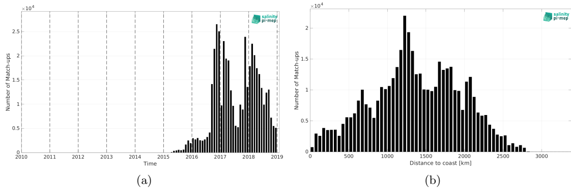
Figure 1: Number of match-ups between Surface drifters and SMAP SSS L2 v5 - 40 km (RSS) SSS as a function of time (a) and as function of the distance to coast (b) over the Pacific Ocean Pi-MEP region and for the full satellite product period.
