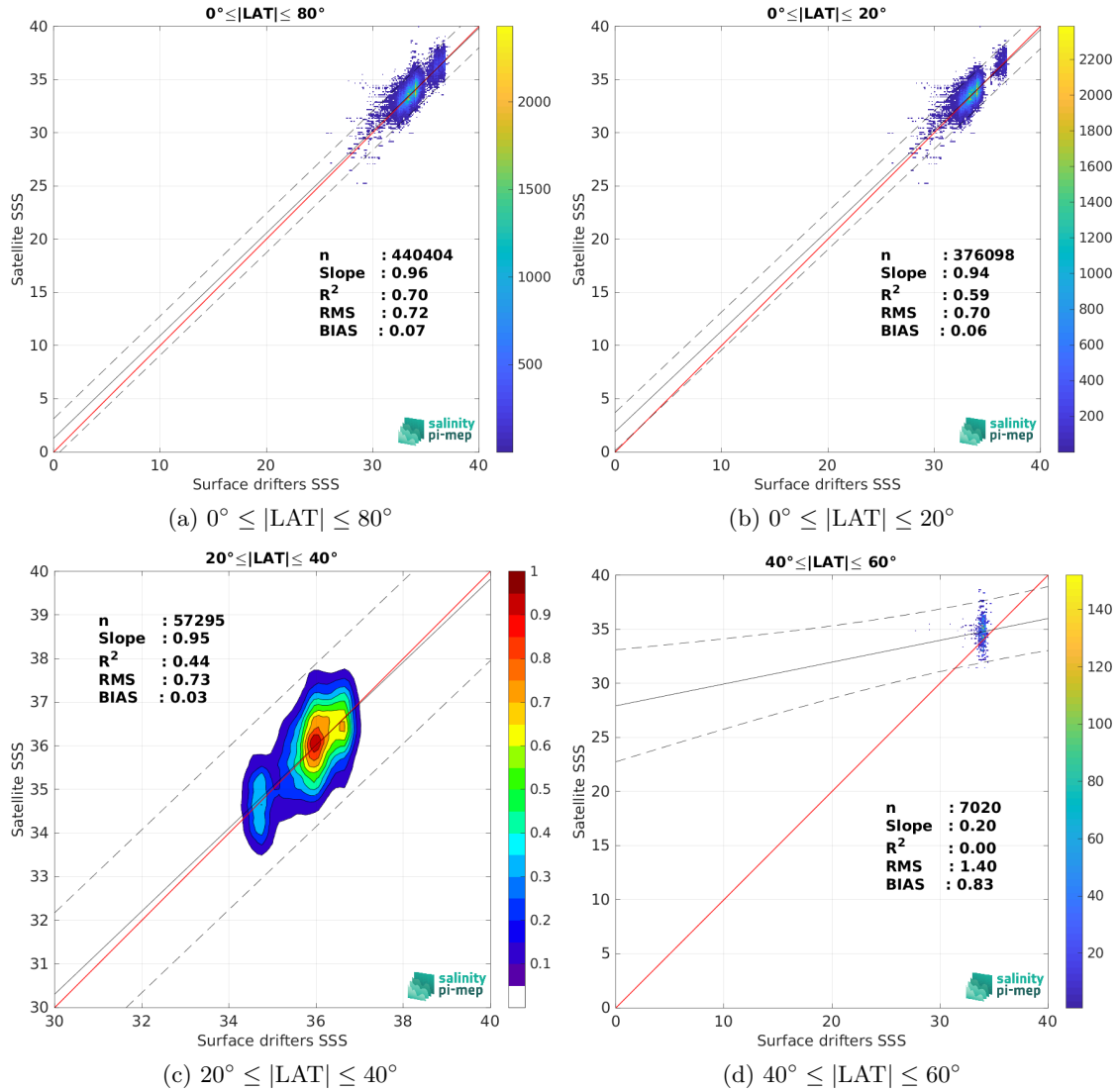
Figure 8: Contour maps of the concentration of SMAP SSS L2 v5 - 40 km (RSS) SSS (y-axis) versus Surface drifters SSS (x-axis) at match-up pairs for different latitude bands. For each plot, the red line shows x=y . The black thin and dashed lines indicate a linear fit through the data cloud and the \pm 95\% confidence levels, respectively. The number match-up pairs n , the slope and R^2 coefficient of the linear fit, the root mean square (RMS) and the mean bias between satellite and in situ data are indicated for each latitude band in each plots.
