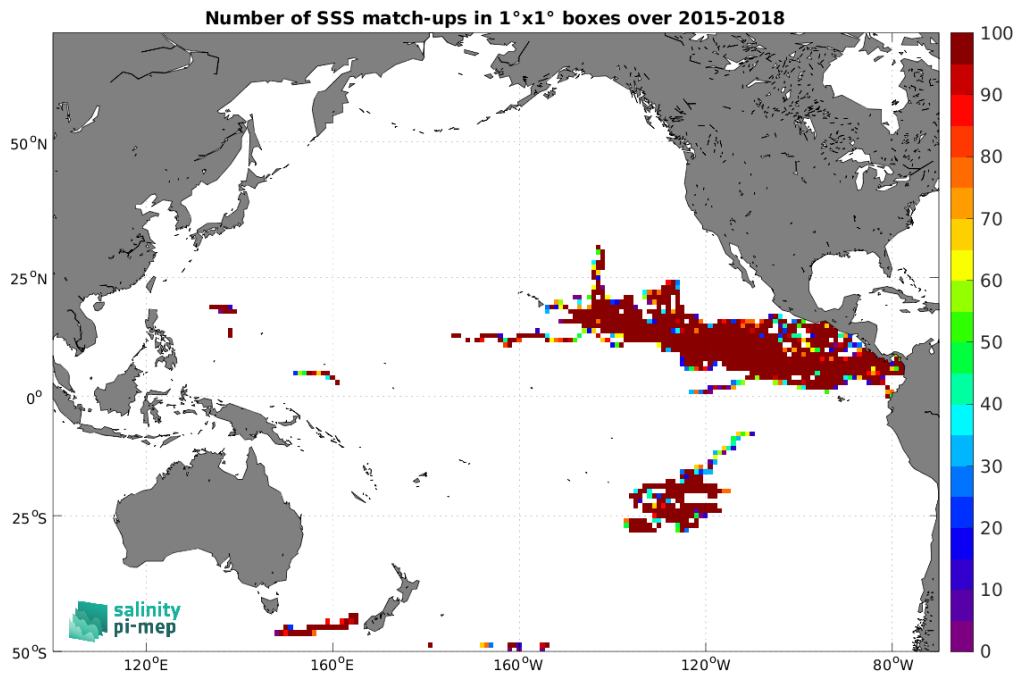
Figure 3: Number of SSS match-ups between Surface drifters SSS and the SMAP SSS L2 v5 - 40 km (RSS) SSS product for the Pacific Ocean Pi-MEP region over 1^\circ \times 1^\circ boxes and for the full satellite product period.
