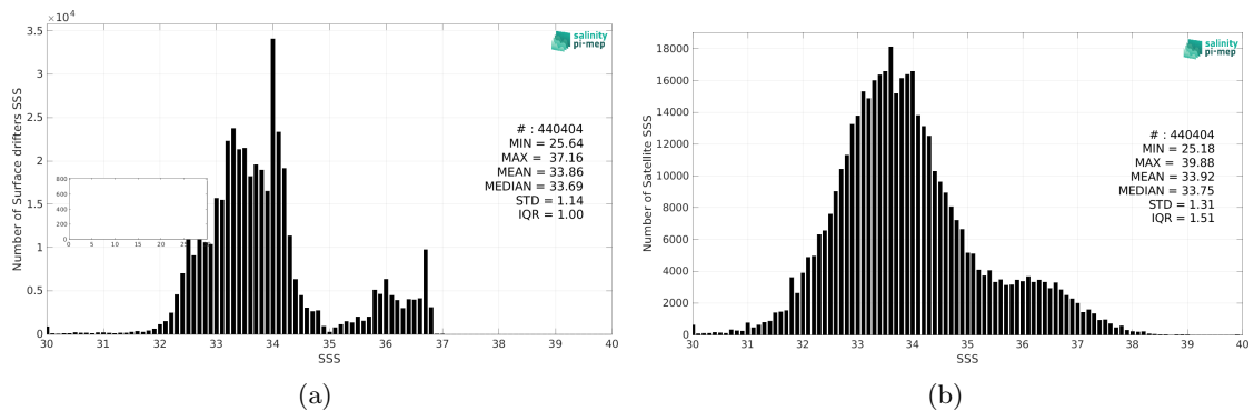
Figure 2: Histograms of SSS from Surface drifters (a) and SMAP SSS L2 v5 - 40 km (RSS) (b) considering all match-up pairs per bins of 0.1 over the Pacific Ocean Pi-MEP region and for the full satellite product period.
