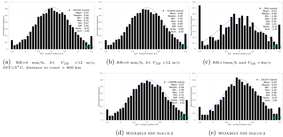
Figure 12: Normalized histogram of \Delta SSS (SMAP SSS L2 v5 - 40 km (RSS) - Surface drifters) for 5 different subdatasets corresponding to: RR=0 mm/h, 3 < U_{10} < 12 m/s, SST > 5°C, distance to coast > 800 km (a), RR=0 mm/h, 3 < U_{10} < 12 m/s (b), RR > 1mm/h and U_{10} < 4 m/s (c), WOA2013 SSS Std < 0.2 (d), WOA2013 SSS Std > 0.2 (e).
