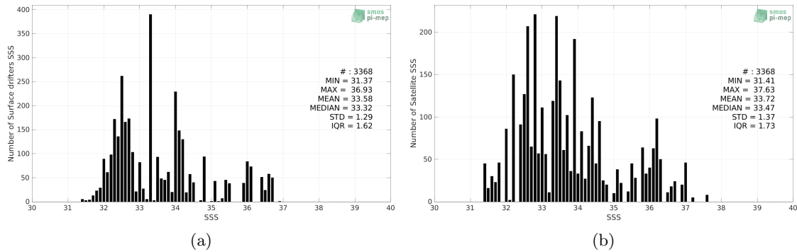
Figure 2: Histograms of SSS from Surface drifters (a) and SMAP SSS L2 v5 - 40 km (RSS) (b) considering all match-up pairs per bins of 0.1 over the Pacific Ocean Pi-MEP region and for the full satellite product period.
