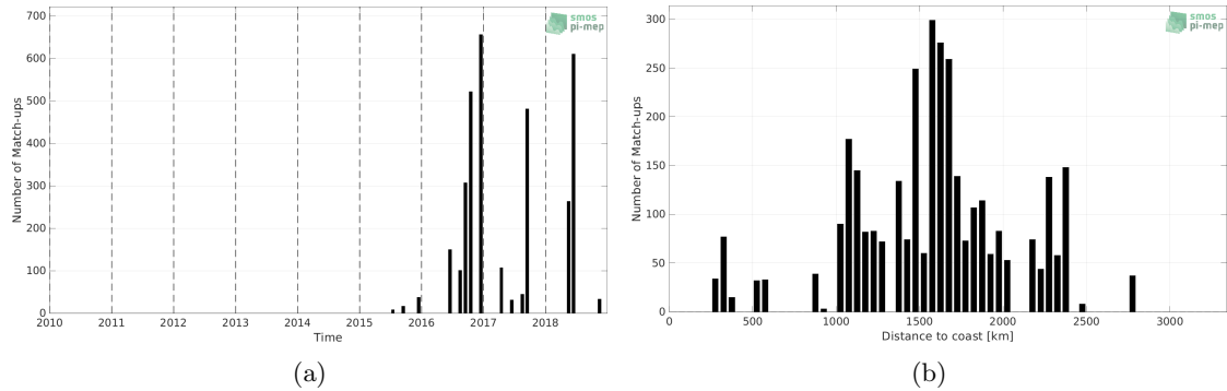
Figure 1: Number of match-ups between Surface drifters and SMAP SSS L2 v5 - 40 km (RSS) SSS as a function of time (a) and as function of the distance to coast (b) over the Pacific Ocean Pi-MEP region and for the full satellite product period.
