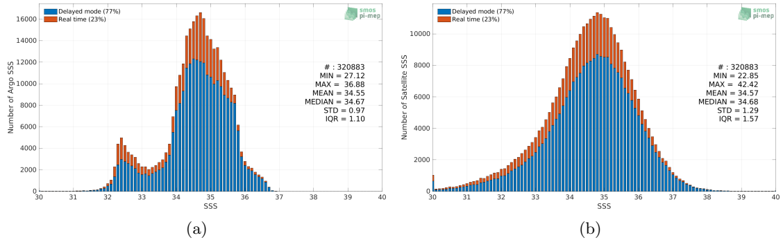
Figure 2: Histograms of SSS from Argo (a) and SMAP SSS L2 v5 - 40 km (RSS) (b) considering all match-up pairs per bins of 0.1 over the Pacific Ocean Pi-MEP region and for the full satellite product period.
