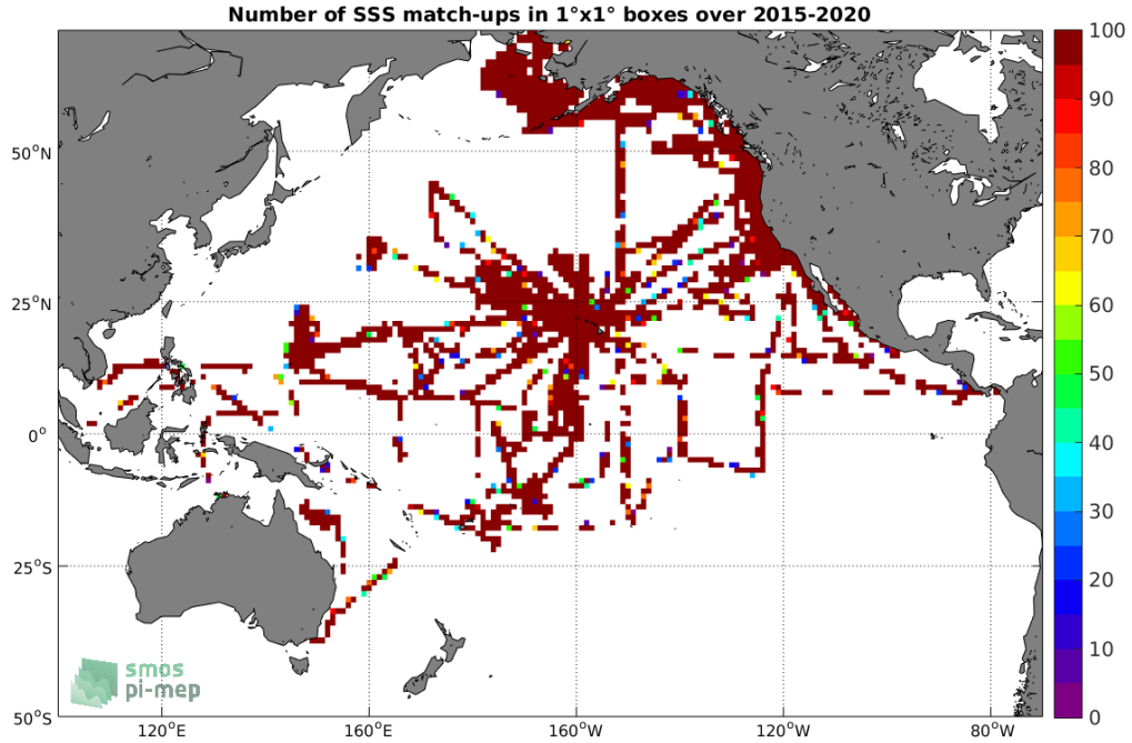
Figure 4: Number of SSS match-ups between TSG (SAMOS) SSS and the SMAP SSS L2 v4 (RSS) SSS product for the Pacific Ocean Pi-MEP region over 1°x1° boxes and for the full satellite product period.
