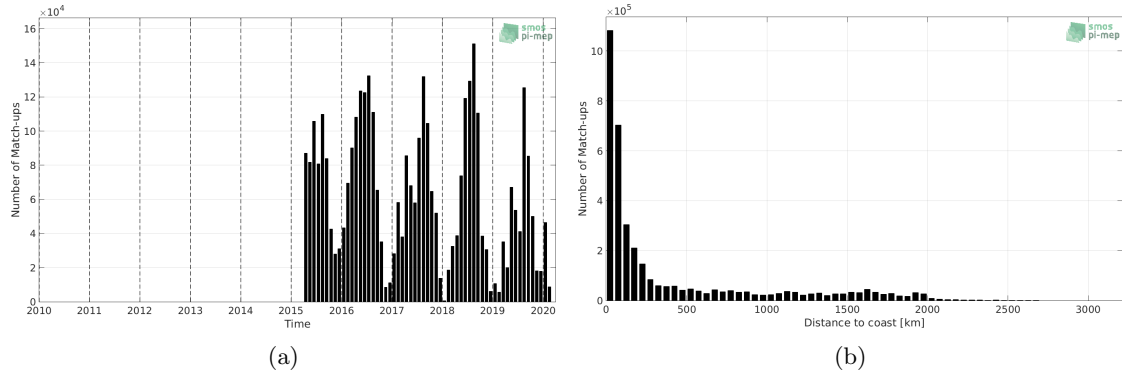
Figure 1: Number of match-ups between TSG-SAMOS and SMAP-L2-RSS-V4 SSS as a function of time (a) and as function of the distance to coast (b) over the Pacific Ocean Pi-MEP region and for the full satellite product period.
