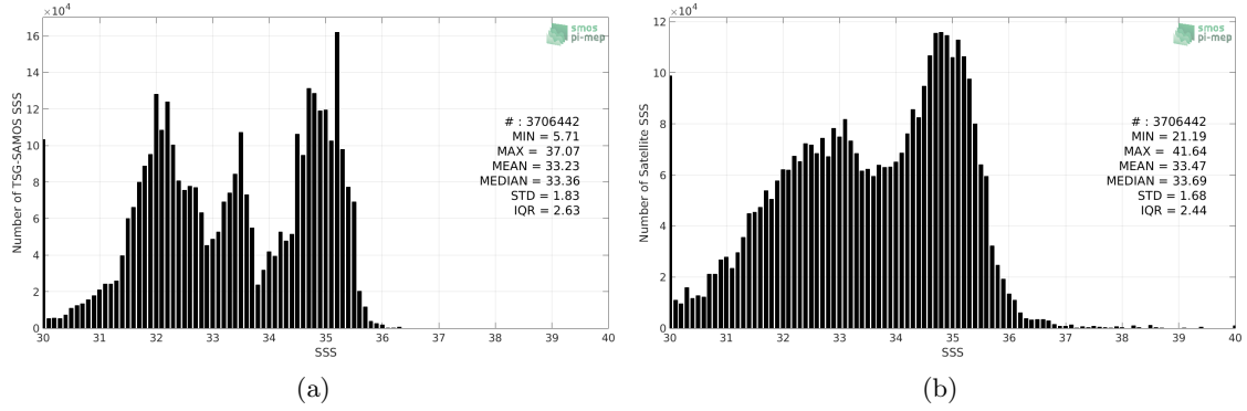
Figure 2: Histograms of SSS from TSG-SAMOS (a) and SMAP-L2-RSS-V4 (b) considering all match-up pairs per bins of 0.1 over the Pacific Ocean Pi-MEP region and for the full satellite product period.
