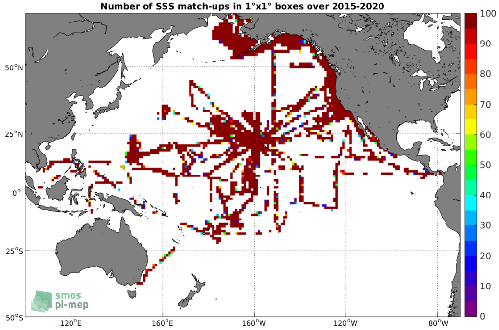
Figure 4: Number of SSS match-ups between TSG-SAMOS SSS and the SMAP-L2-RSS-V4 SSS product for the Pacific Ocean Pi-MEP region over 1^\circ \times 1^\circ boxes and for the full satellite product period.
