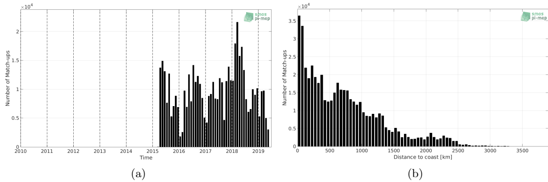
Figure 1: Number of match-ups between TSG-LEGOS-DM and SMAP-L2-RSS-V4 SSS as a function of time (a) and as function of the distance to coast (b) over the Pacific Ocean Pi-MEP region and for the full satellite product period.
