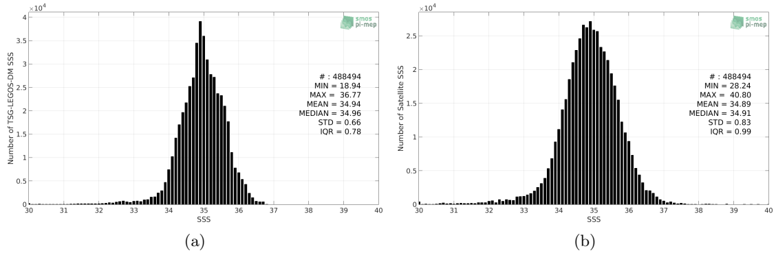
Figure 2: Histograms of SSS from TSG-LEGOS-DM (a) and SMAP-L2-RSS-V4 (b) considering all match-up pairs per bins of 0.1 over the Pacific Ocean Pi-MEP region and for the full satellite product period.
