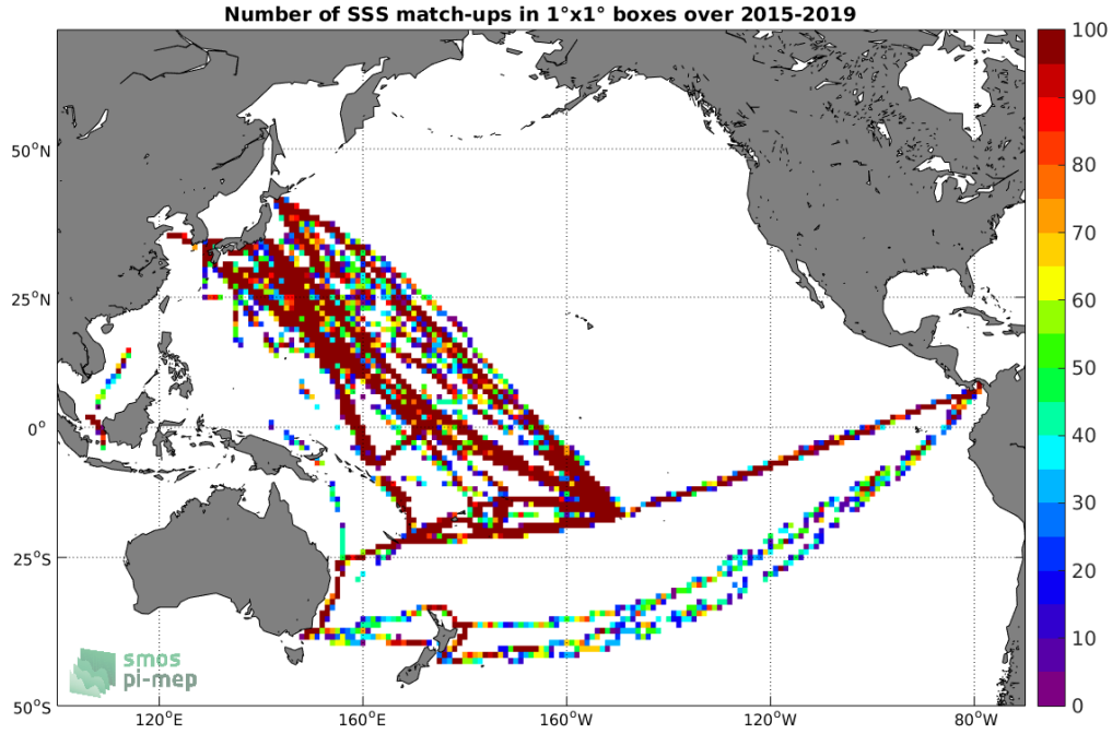
Figure 4: Number of SSS match-ups between TSG-LEGOS-DM SSS and the SMAP-L2-RSS-V4 SSS product for the Pacific Ocean Pi-MEP region over 1^\circ \times 1^\circ boxes and for the full satellite product period.
