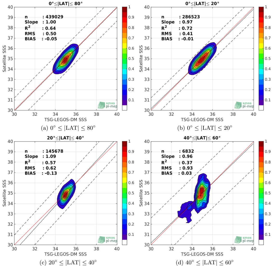
Figure 9: Contour maps of the concentration of SMAP-L2-RSS-V4 SSS (y-axis) versus TSG-LEGOS-DM SSS (x-axis) at match-up pairs for different latitude bands. For each plot, the red line shows x=y . The black thin and dashed lines indicate a linear fit through the data cloud and the \pm 95\% confidence levels, respectively. The number match-up pairs n , the slope and R^2 coefficient of the linear fit, the root mean square (RMS) and the mean bias between satellite and in situ data are indicated for each latitude band in each plots.
