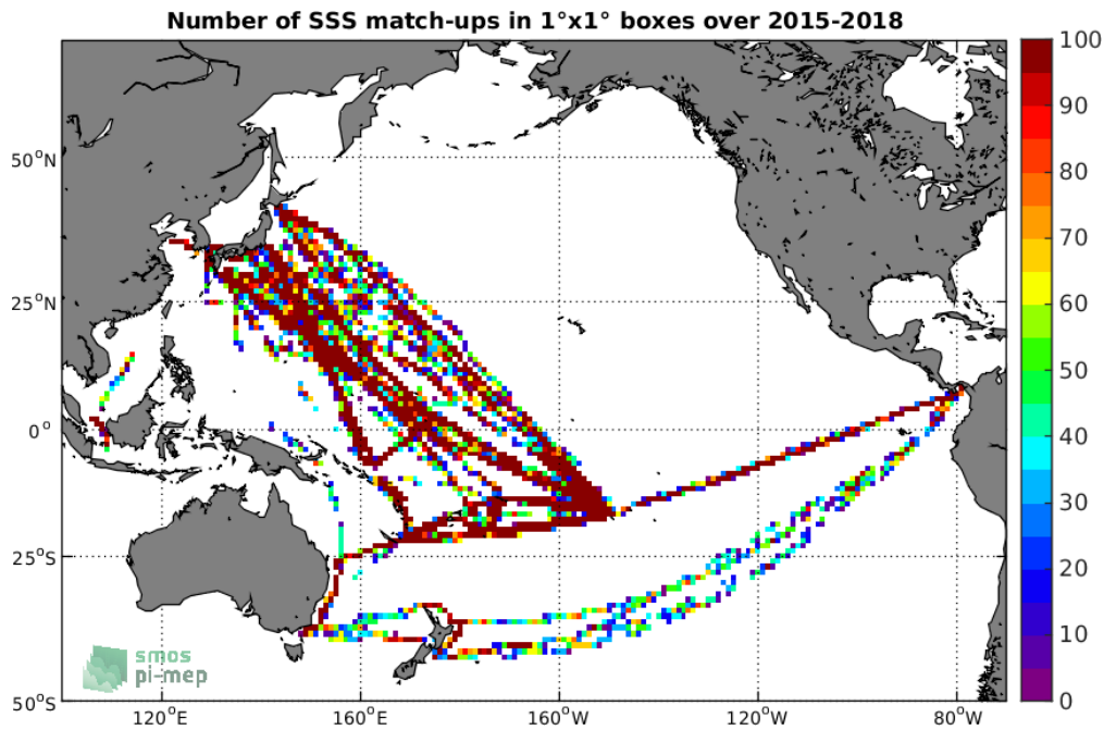
Figure 4: Number of SSS match-ups between TSG-LEGOS-DM SSS and the SMAP-L2-RSS-V4 SSS product for the Pacific Ocean Pi-MEP region over 1°x1° boxes and for the full satellite product period.
