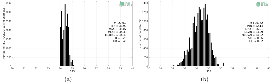
Figure 2: Histograms of SSS from TSG (GOSUD-Sailing-ship) (a) and SMAP SSS L2 v4 (RSS) (b) considering all match-up pairs per bins of 0.1 over the Pacific Ocean Pi-MEP region and for the full satellite product period.
