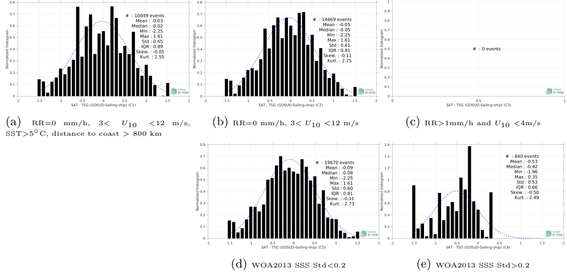
Figure 13: Normalized histogram of \Delta SSS (SMAP SSS L2 v4 (RSS) - TSG (GOSUD-Sailing-ship)) for 5 different subdatasets corresponding to: RR=0 mm/h, 3 < U_{10} < 12 m/s, SST>5°C, distance to coast > 800 km (a), RR=0 mm/h, 3 < U_{10} < 12 m/s (b), RR>1mm/h and U_{10} < 4 m/s (c), WOA2013 SSS Std<0.2 (d), WOA2013 SSS Std>0.2 (e).
