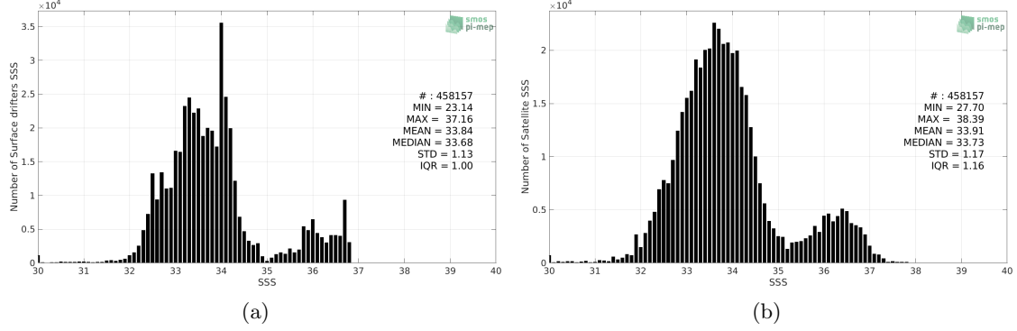
Figure 2: Histograms of SSS from Surface drifters (a) and SMAP SSS L2 v4 (RSS) (b) considering all match-up pairs per bins of 0.1 over the Pacific Ocean Pi-MEP region and for the full satellite product period.
