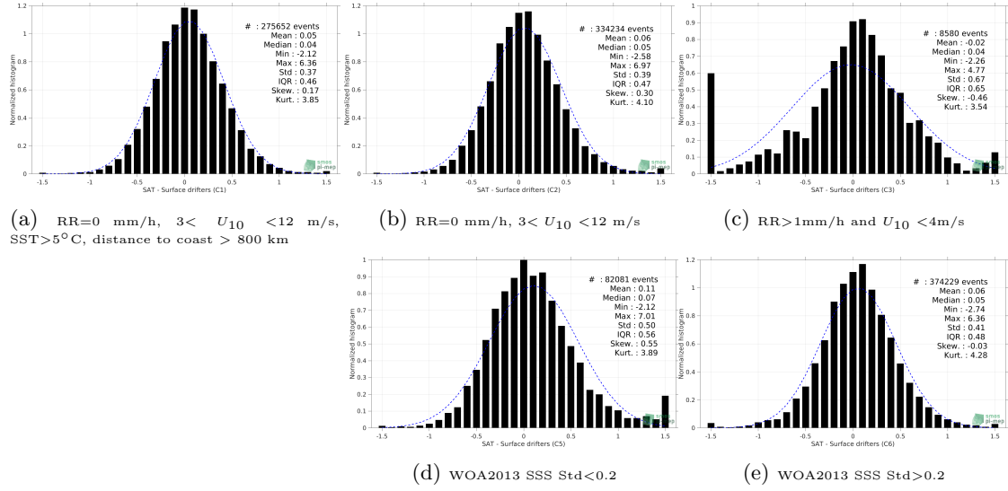
Figure 12: Normalized histogram of \Delta\text{SSS} (SMAP SSS L2 v4 (RSS) - Surface drifters) for 5 different subdatasets corresponding to: RR=0 mm/h, 3 < U_{10} < 12 m/s, SST>5°C, distance to coast > 800 km (a), RR=0 mm/h, 3 < U_{10} < 12 m/s (b), RR>1mm/h and U_{10} < 4 m/s (c), WOA2013 SSS Std<0.2 (d), WOA2013 SSS Std>0.2 (e).
