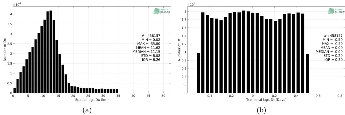
Figure 4: Histograms of the spatial (a) and temporal (b) lags between the location/time of the Surface drifters measurement and the date of the corresponding SMAP SSS L2 v4 (RSS) SSS pixel.
