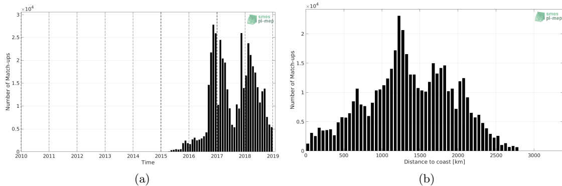
Figure 1: Number of match-ups between Surface drifters and SMAP SSS L2 v4 (RSS) SSS as a function of time (a) and as function of the distance to coast (b) over the Pacific Ocean Pi-MEP region and for the full satellite product period.
