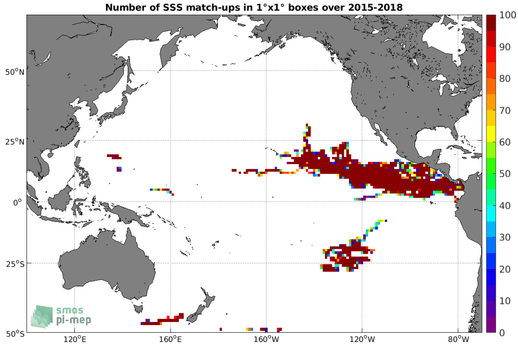
Figure 3: Number of SSS match-ups between Surface drifters SSS and the SMAP SSS L2 v4 (RSS) SSS product for the Pacific Ocean Pi-MEP region over 1^\circ \times 1^\circ boxes and for the full satellite product period.
