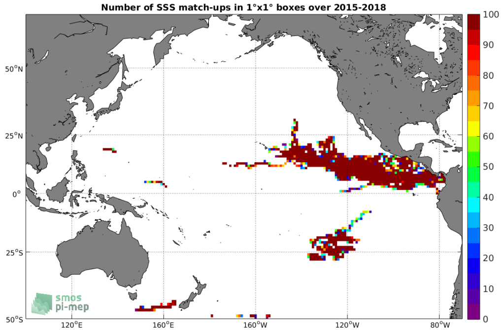
Figure 3: Number of SSS match-ups between Surface drifters SSS and the SMAP SSS L2 v4 (RSS) SSS product for the Pacific Ocean Pi-MEP region over 1°x1° boxes and for the full satellite product period.
