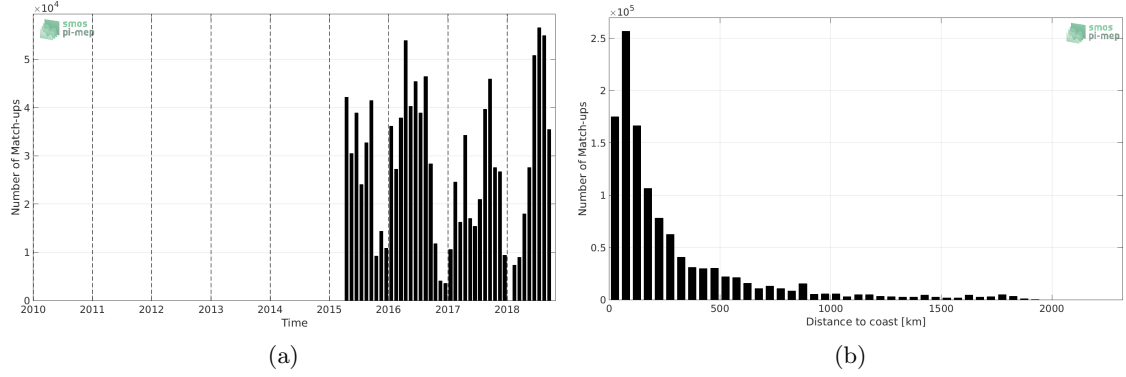
Figure 1: Number of match-ups between TSG-SAMOS and SMAP-L2-RSS-V3-70KM SSS as a function of time (a) and as function of the distance to coast (b) over the Pacific Ocean Pi-MEP region and for the full satellite product period.
