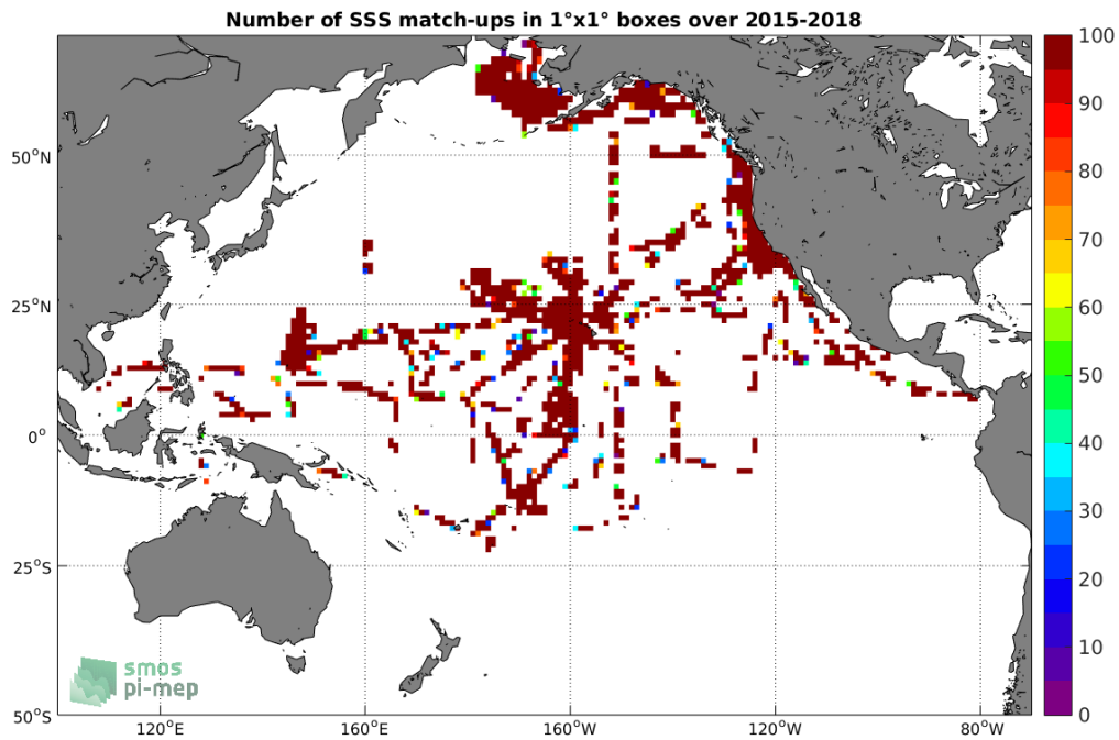
Figure 4: Number of SSS match-ups between TSG-SAMOS SSS and the SMAP-L2-RSS-V3-70KM SSS product for the Pacific Ocean Pi-MEP region over 1^\circ \times 1^\circ boxes and for the full satellite product period.
