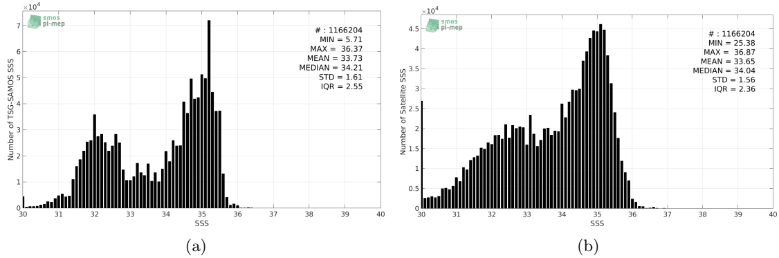
Figure 2: Histograms of SSS from TSG-SAMOS (a) and SMAP-L2-RSS-V3-70KM (b) considering all match-up pairs per bins of 0.1 over the Pacific Ocean Pi-MEP region and for the full satellite product period.
