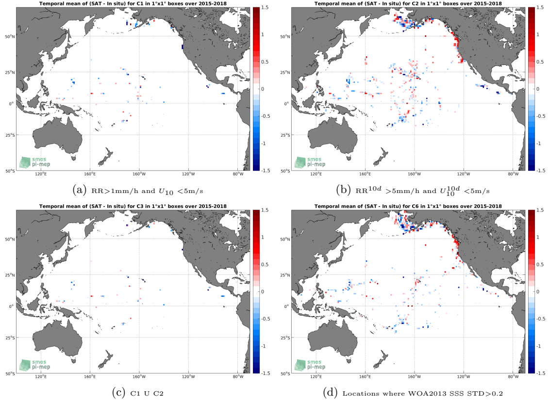
Figure 12: Temporal mean gridded over spatial boxes of size 1^\circ \times 1^\circ of \Delta SSS (SMAP-L2-RSS-V3-70KM - TSG-SAMOS) for 4 different subdatasets corresponding to: RR > 1\text{mm/h} and U_{10} < 5\text{m/s} (a), RR^{10d} > 5\text{mm/h} and U_{10}^{10d} < 5\text{m/s} (b), C1 U C2 (c), Locations where WOA2013 SSS STD > 0.2 (d).
