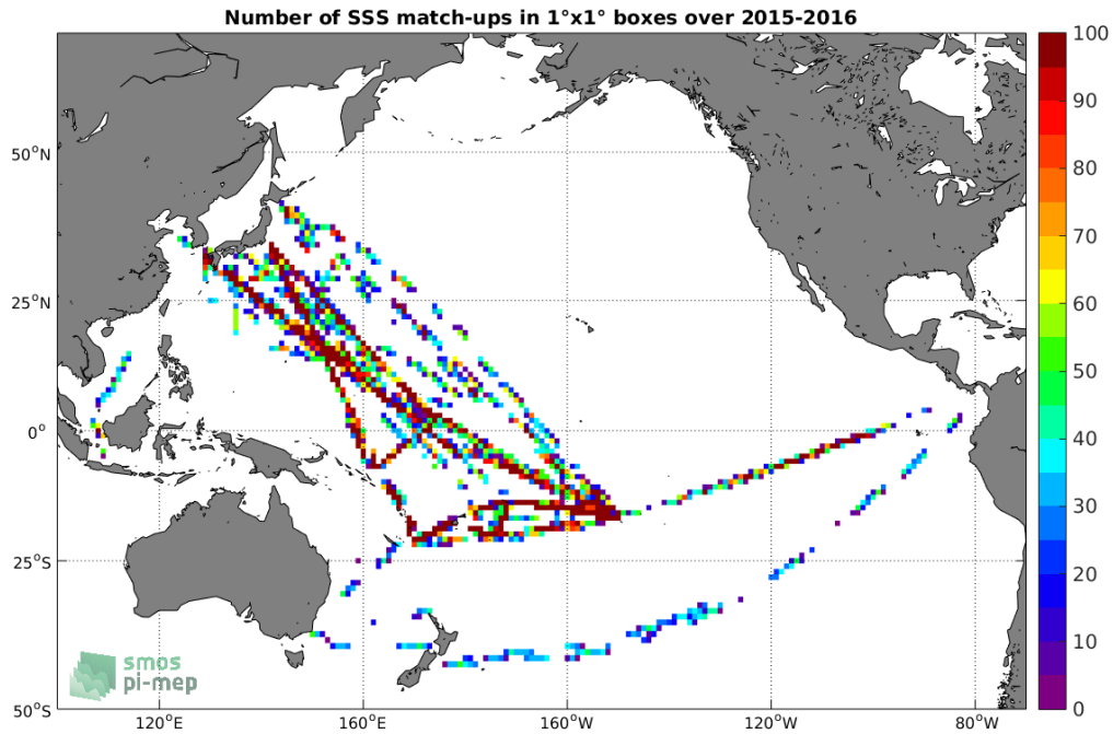
Figure 4: Number of SSS match-ups between TSG-LEGOS-DM SSS and the SMAP-L2-RSS-V3-70KM SSS product for the Pacific Ocean Pi-MEP region over 1^\circ \times 1^\circ boxes and for the full satellite product period.
