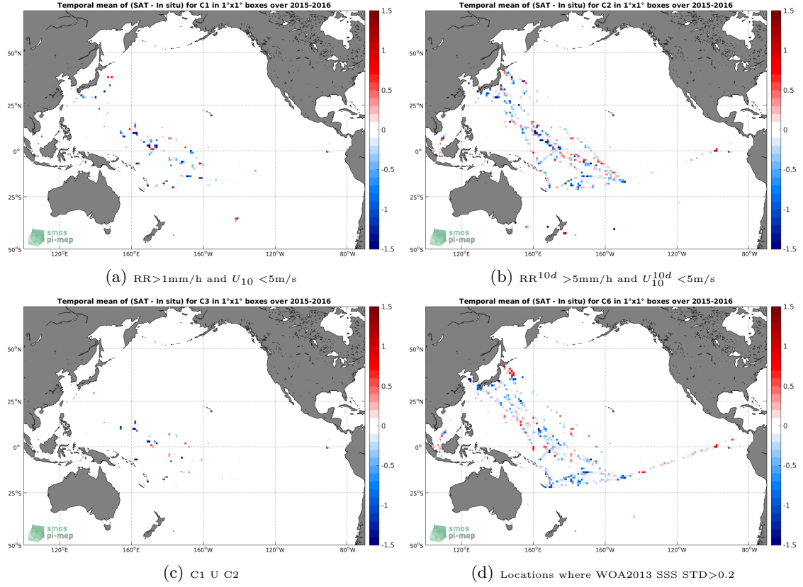
Figure 12: Temporal mean gridded over spatial boxes of size 1^\circ \times 1^\circ of \Delta SSS (SMAP-L2-RSS-V3-70KM - TSG-LEGOS-DM) for 4 different subdatasets corresponding to: RR > 1mm/h and U_{10} < 5\text{m/s} (a), RR^{10d} > 5\text{mm/h} and U_{10}^{10d} < 5\text{m/s} (b), C1 U C2 (c), Locations where WOA2013 SSS STD > 0.2 (d).
