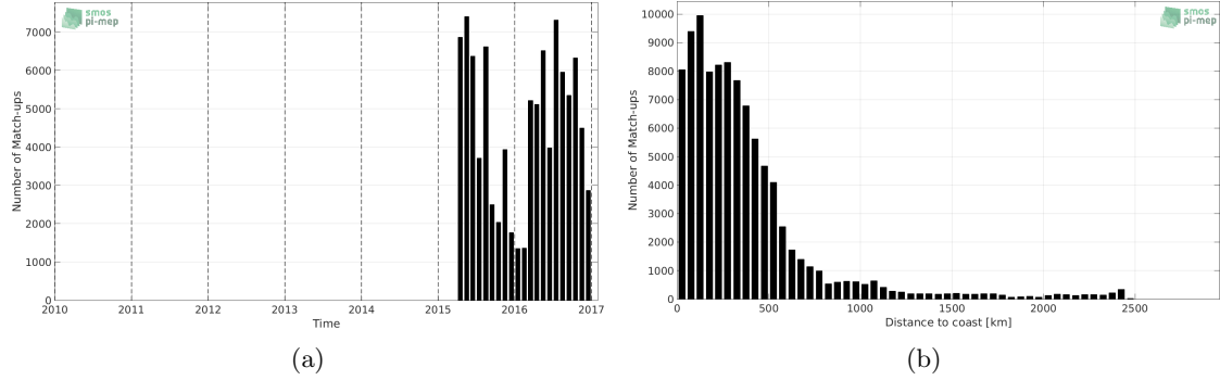
Figure 1: Number of match-ups between TSG-LEGOS-DM and SMAP-L2-RSS-V3-70KM SSS as a function of time (a) and as function of the distance to coast (b) over the Pacific Ocean Pi-MEP region and for the full satellite product period.
