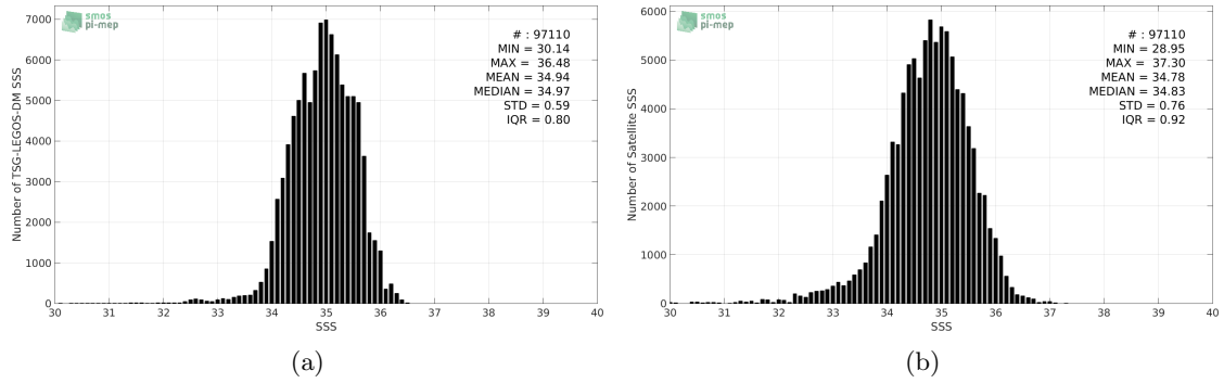
Figure 2: Histograms of SSS from TSG-LEGOS-DM (a) and SMAP-L2-RSS-V3-70KM (b) considering all match-up pairs per bins of 0.1 over the Pacific Ocean Pi-MEP region and for the full satellite product period.
