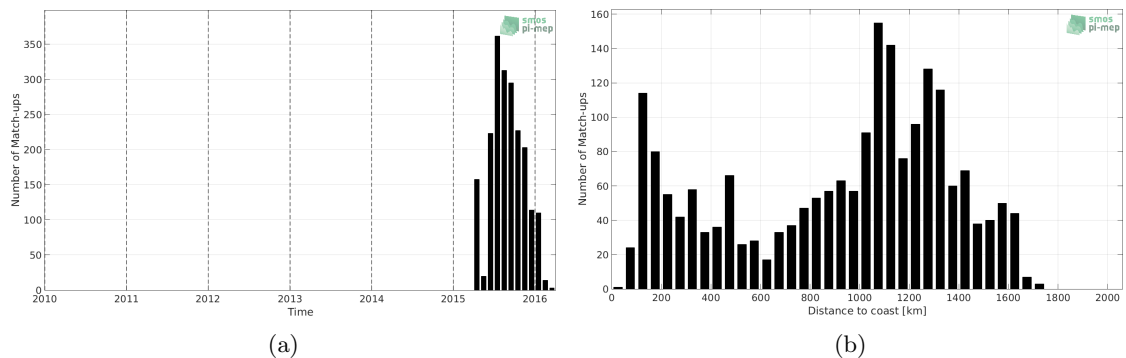
Figure 1: Number of match-ups between Sea mammals and SMAP-L2-RSS-V3-70KM SSS as a function of time (a) and as function of the distance to coast (b) over the Pacific Ocean Pi-MEP region and for the full satellite product period.
