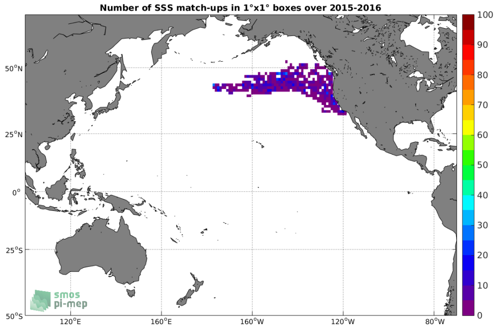
Figure 4: Number of SSS match-ups between Sea mammals SSS and the SMAP-L2-RSS-V3-70KM SSS product for the Pacific Ocean Pi-MEP region over 1°x1° boxes and for the full satellite product period.
