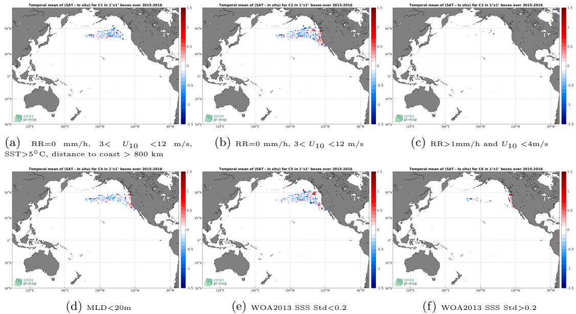
Figure 12: Temporal mean gridded over spatial boxes of size 1^\circ \times 1^\circ of \Delta SSS (SMAP-L2-RSS-V3-70KM - Sea mammals) for 6 different subdatasets corresponding to:RR=0 mm/h, 3 < U_{10} < 12 m/s, SST >5^\circ C, distance to coast > 800 km (a), RR=0 mm/h, 3 < U_{10} < 12 m/s (b), RR >1 mm/h and U_{10} < 4 m/s (c),MLD <20 m (d),WOA2013 SSS Std <0.2 (e),WOA2013 SSS Std >0.2 (f).
