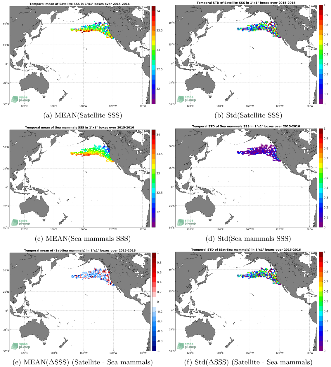
Figure 6: Temporal mean (left) and Std (right) of SSS from SMAP-L2-RSS-V3-70KM (top), Sea mammals (middle), and of \Delta SSS (Satellite - Sea mammals). Only match-up pairs are used to generate these maps.
