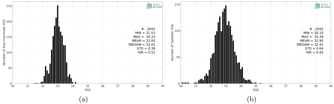
Figure 2: Histograms of SSS from Sea mammals (a) and SMAP-L2-RSS-V3-70KM (b) considering all match-up pairs per bins of 0.1 over the Pacific Ocean Pi-MEP region and for the full satellite product period.
