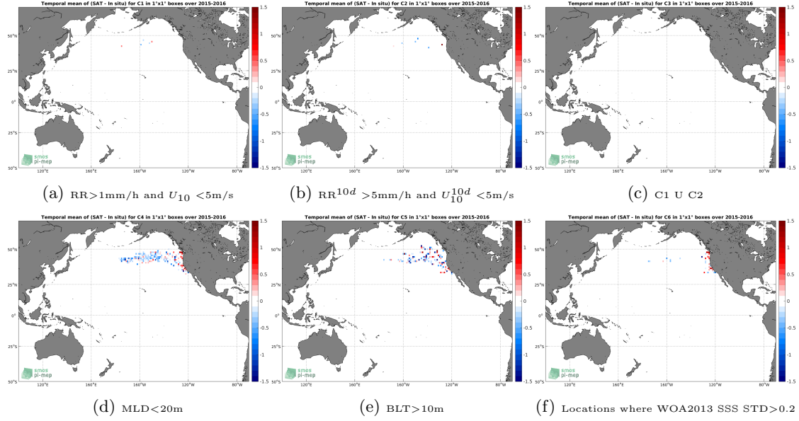
Figure 12: Temporal mean gridded over spatial boxes of size 1^\circ \times 1^\circ of \Delta\text{SSS} (SMAP-L2-RSS-V3-70KM - Sea mammals) for 6 different subdatasets corresponding to: \text{RR} > 1\text{mm/h} and U_{10} < 5\text{m/s} (a), \text{RR}^{10d} > 5\text{mm/h} and U_{10}^{10d} < 5\text{m/s} (b), C1 U C2 (c), \text{MLD} < 20\text{m} (d), \text{BLT} > 10\text{m} (e), Locations where WOA2013 SSS STD > 0.2 (f).
