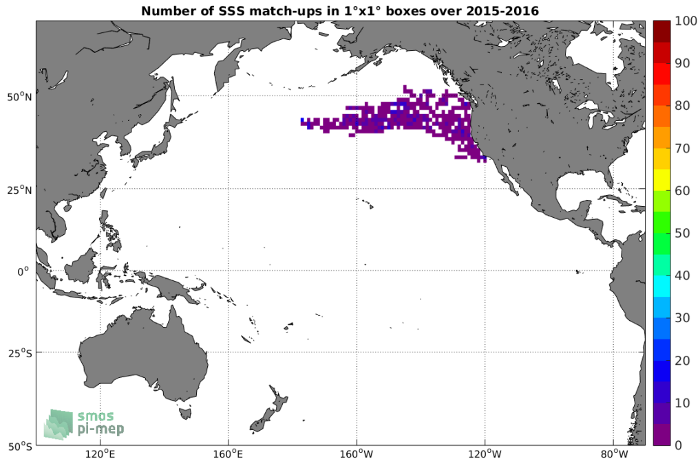
Figure 4: Number of SSS match-ups between Sea mammals SSS and the SMAP-L2-RSS-V3-70KM SSS product for the Pacific Ocean Pi-MEP region over 1^\circ \times 1^\circ boxes and for the full satellite product period.
