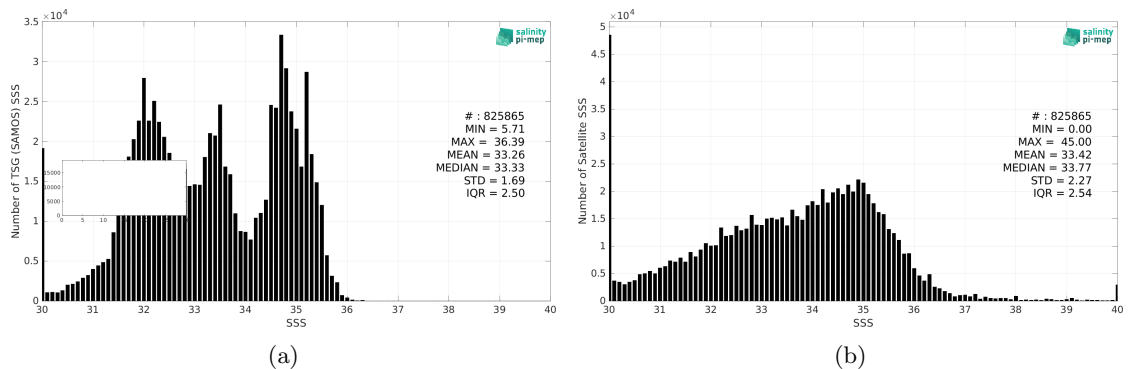
Figure 2: Histograms of SSS from TSG (SAMOS) (a) and SMAP SSS L2 v5.0 (JPL) (b) considering all match-up pairs per bins of 0.1 over the Pacific Ocean Pi-MEP region and for the full satellite product period.
