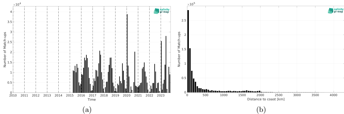
Figure 1: Number of match-ups between TSG (SAMOS) and SMAP SSS L2 v5.0 (JPL) SSS as a function of time (a) and as function of the distance to coast (b) over the Pacific Ocean Pi-MEP region and for the full satellite product period.
