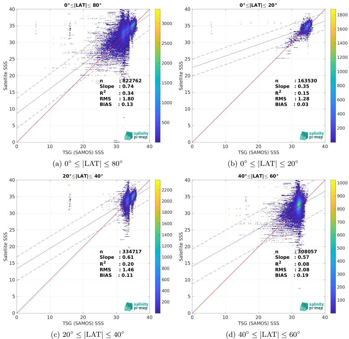
Figure 9: Contour maps of the concentration of SMAP SSS L2 v5.0 (JPL) SSS (y-axis) versus TSG (SAMOS) SSS (x-axis) at match-up pairs for different latitude bands. For each plot, the red line shows x=y . The black thin and dashed lines indicate a linear fit through the data cloud and the \pm 95\% confidence levels, respectively. The number match-up pairs n , the slope and R^2 coefficient of the linear fit, the root mean square (RMS) and the mean bias between satellite and in situ data are indicated for each latitude band in each plots.
