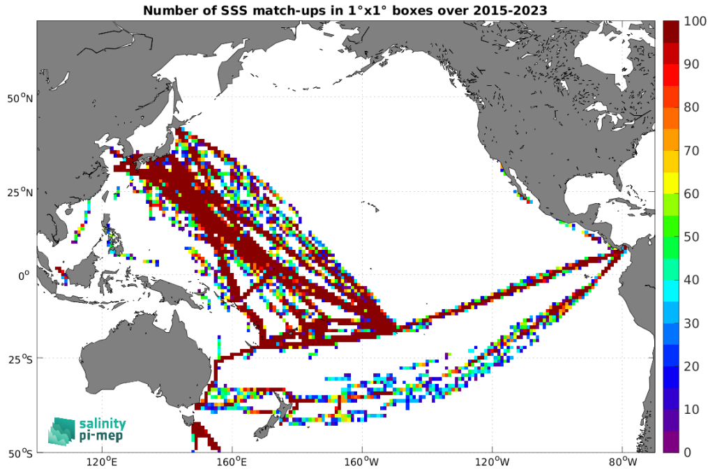
Figure 5: Number of SSS match-ups between TSG (LEGOS-DM) SSS and the SMAP SSS L2 v5.0 (JPL) SSS product for the Pacific Ocean Pi-MEP region over 1^\circ \times 1^\circ boxes and for the full satellite product period.
