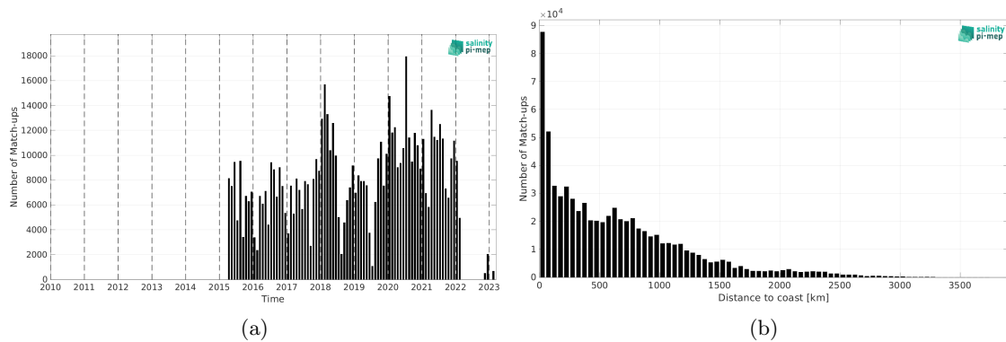
Figure 2: Number of match-ups between TSG (LEGOS-DM) and SMAP SSS L2 v5.0 (JPL) SSS as a function of time (a) and as function of the distance to coast (b) over the Pacific Ocean Pi-MEP region and for the full satellite product period.
