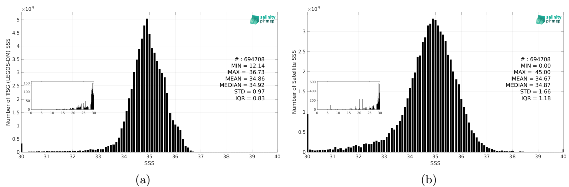
Figure 3: Histograms of SSS from TSG (LEGOS-DM) (a) and SMAP SSS L2 v5.0 (JPL) (b) considering all match-up pairs per bins of 0.1 over the Pacific Ocean Pi-MEP region and for the full satellite product period.
