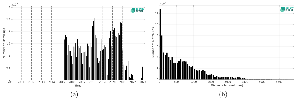
Figure 1: Number of match-ups between TSG (LEGOS-DM) and SMAP SSS L2 v5.0 (JPL) SSS as a function of time (a) and as function of the distance to coast (b) over the Pacific Ocean Pi-MEP region and for the full satellite product period.
