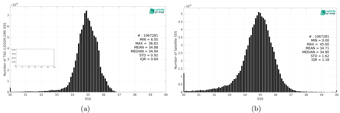
Figure 2: Histograms of SSS from TSG (LEGOS-DM) (a) and SMAP SSS L2 v5.0 (JPL) (b) considering all match-up pairs per bins of 0.1 over the Pacific Ocean Pi-MEP region and for the full satellite product period.
