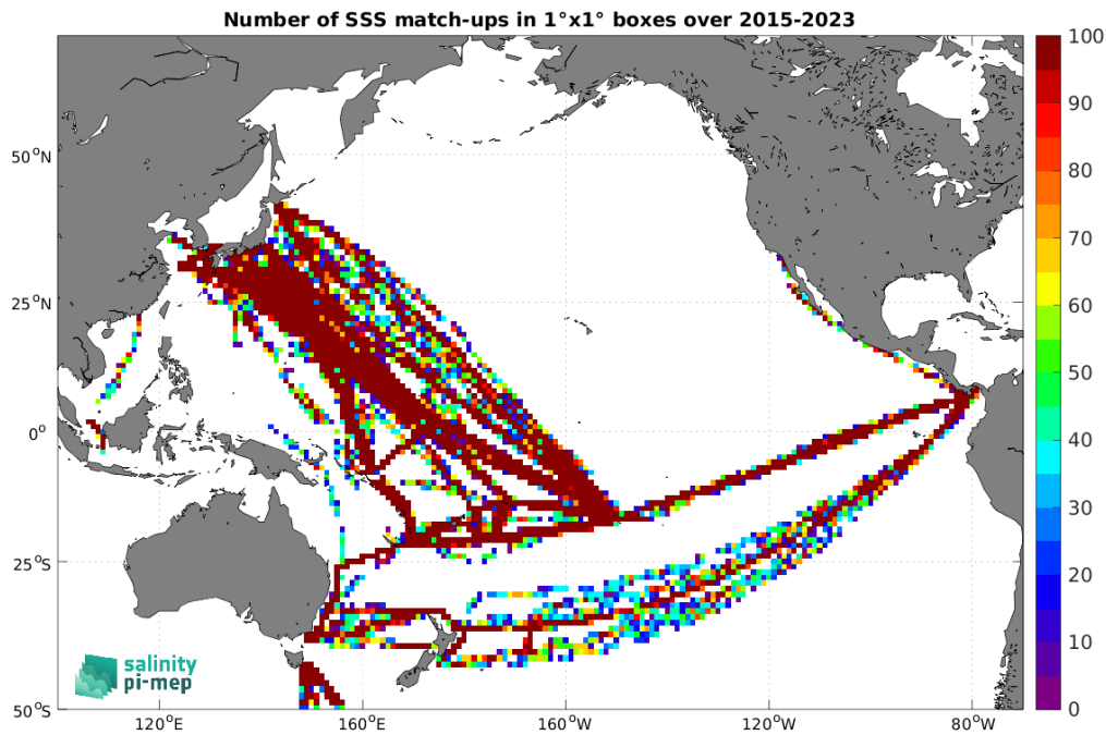
Figure 4: Number of SSS match-ups between TSG (LEGOS-DM) SSS and the SMAP SSS L2 v5.0 (JPL) SSS product for the Pacific Ocean Pi-MEP region over 1^\circ \times 1^\circ boxes and for the full satellite product period.
