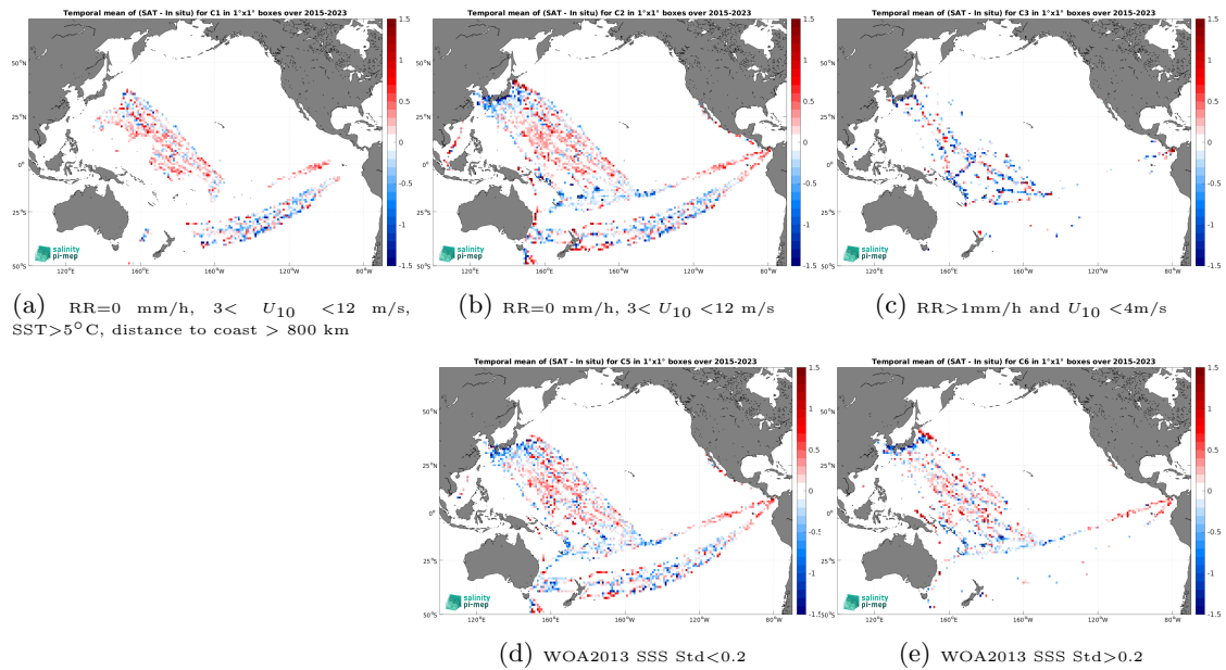
Figure 12: Temporal mean gridded over spatial boxes of size 1^\circ \times 1^\circ of \Delta\text{SSS} (SMAP SSS L2 v5.0 (JPL) - TSG (LEGOS-DM)) for 5 different subdatasets corresponding to:RR=0 mm/h, 3 < U_{10} < 12 m/s, SST >5^\circ\text{C} , distance to coast > 800 km (a), RR=0 mm/h, 3 < U_{10} < 12 m/s (b), RR >1 mm/h and U_{10} < 4 m/s (c), WOA2013 SSS Std <0.2 (d), WOA2013 SSS Std >0.2 (e).
