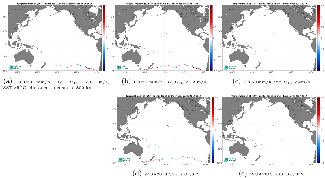
Figure 14: Temporal mean gridded over spatial boxes of size 1^\circ \times 1^\circ of \Delta SSS (SMAP SSS L2 v5.0 (JPL) - TSG (GOSUD-Sailing-ship)) for 5 different subdatasets corresponding to:RR=0 mm/h, 3 < U_{10} < 12 m/s, SST>5°C, distance to coast > 800 km (a), RR=0 mm/h, 3 < U_{10} < 12 m/s (b), RR>1mm/h and U_{10} < 4 m/s (c), WOA2013 SSS Std<0.2 (d), WOA2013 SSS Std>0.2 (e).
