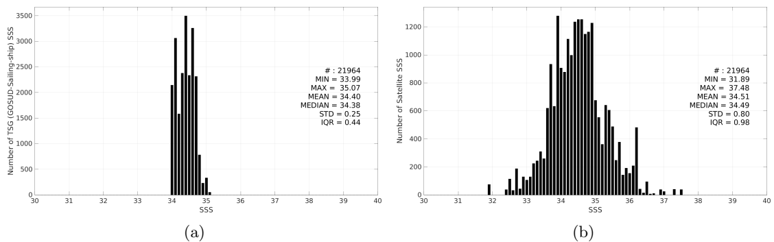
Figure 3: Histograms of SSS from TSG (GOSUD-Sailing-ship) (a) and SMAP SSS L2 v5.0 (JPL) (b) considering all match-up pairs per bins of 0.1 over the Pacific Ocean Pi-MEP region and for the full satellite product period.
