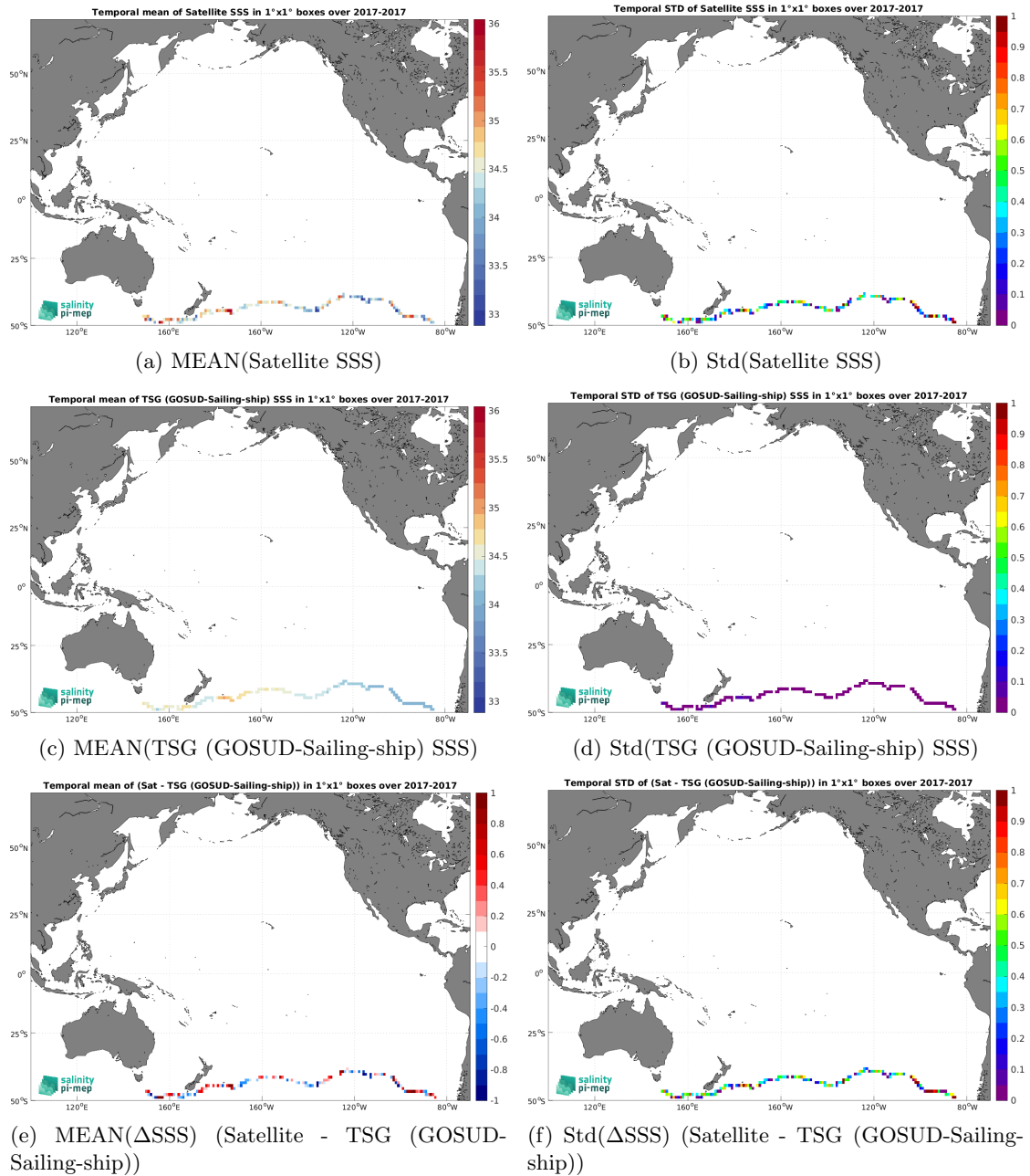
Figure 7: Temporal mean (left) and Std (right) of SSS from SMAP SSS L2 v5.0 (JPL) (top), TSG (GOSUD-Sailing-ship) (middle), and of \Delta SSS (Satellite - TSG (GOSUD-Sailing-ship)). Only match-up pairs are used to generate these maps.
