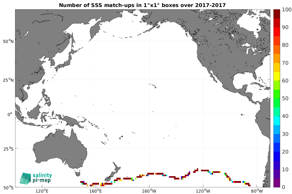
Figure 5: Number of SSS match-ups between TSG (GOSUD-Sailing-ship) SSS and the SMAP SSS L2 v5.0 (JPL) SSS product for the Pacific Ocean Pi-MEP region over 1^\circ \times 1^\circ boxes and for the full satellite product period.
