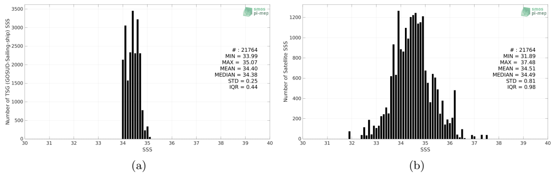
Figure 2: Histograms of SSS from TSG (GOSUD-Sailing-ship) (a) and SMAP SSS L2 v5.0 (JPL) (b) considering all match-up pairs per bins of 0.1 over the Pacific Ocean Pi-MEP region and for the full satellite product period.
