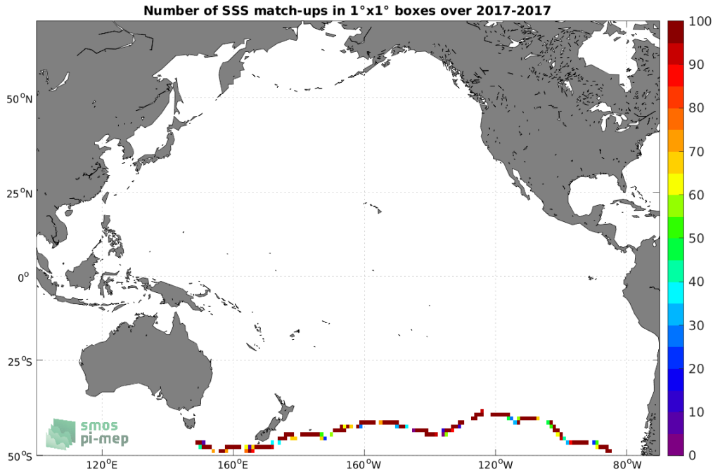
Figure 4: Number of SSS match-ups between TSG (GOSUD-Sailing-ship) SSS and the SMAP SSS L2 v5.0 (JPL) SSS product for the Pacific Ocean Pi-MEP region over 1^\circ \times 1^\circ boxes and for the full satellite product period.
