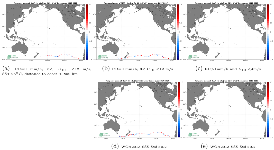
Figure 12: Temporal mean gridded over spatial boxes of size 1^\circ \times 1^\circ of \Delta SSS (SMAP SSS L2 v5.0 (JPL) - TSG (GOSUD-Sailing-ship)) for 5 different subdatasets corresponding to: RR=0 mm/h, 3 < U_{10} < 12 m/s, SST > 5°C, distance to coast > 800 km (a), RR=0 mm/h, 3 < U_{10} < 12 m/s (b), RR > 1mm/h and U_{10} < 4 m/s (c), WOA2013 SSS Std < 0.2 (d), WOA2013 SSS Std > 0.2 (e).
