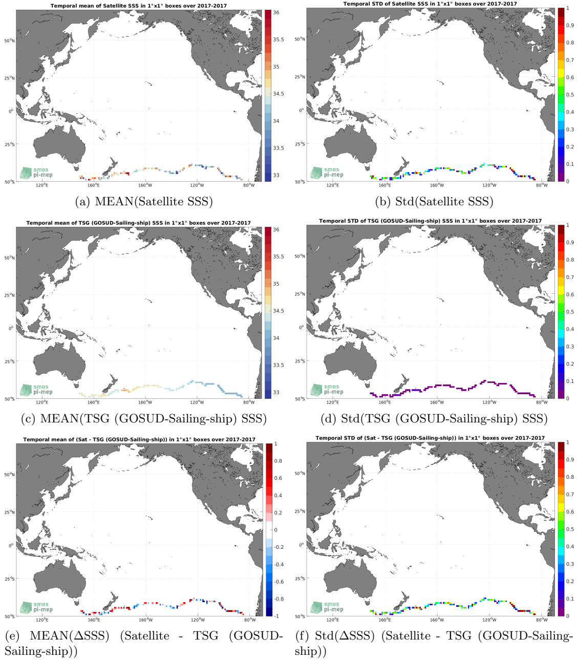
Figure 6: Temporal mean (left) and Std (right) of SSS from SMAP SSS L2 v5.0 (JPL) (top), TSG (GOSUD-Sailing-ship) (middle), and of \Delta SSS (Satellite - TSG (GOSUD-Sailing-ship)). Only match-up pairs are used to generate these maps.
