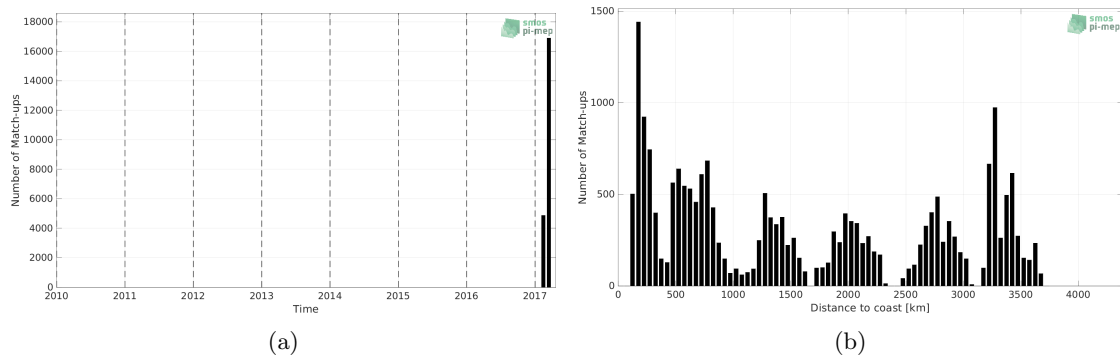
Figure 1: Number of match-ups between TSG (GOSUD-Sailing-ship) and SMAP SSS L2 v5.0 (JPL) SSS as a function of time (a) and as function of the distance to coast (b) over the Pacific Ocean Pi-MEP region and for the full satellite product period.
