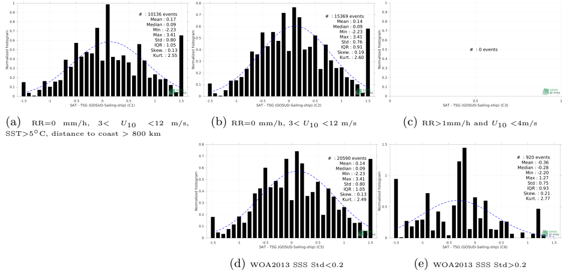
Figure 13: Normalized histogram of \Delta SSS (SMAP SSS L2 v5.0 (JPL) - TSG (GOSUD-Sailing-ship)) for 5 different subdatasets corresponding to: RR=0 mm/h, 3 < U_{10} < 12 m/s, SST >5^{\circ} C, distance to coast > 800 km (a), RR=0 mm/h, 3 < U_{10} < 12 m/s (b), RR >1 mm/h and U_{10} < 4 m/s (c), WOA2013 SSS Std <0.2 (d), WOA2013 SSS Std >0.2 (e).
